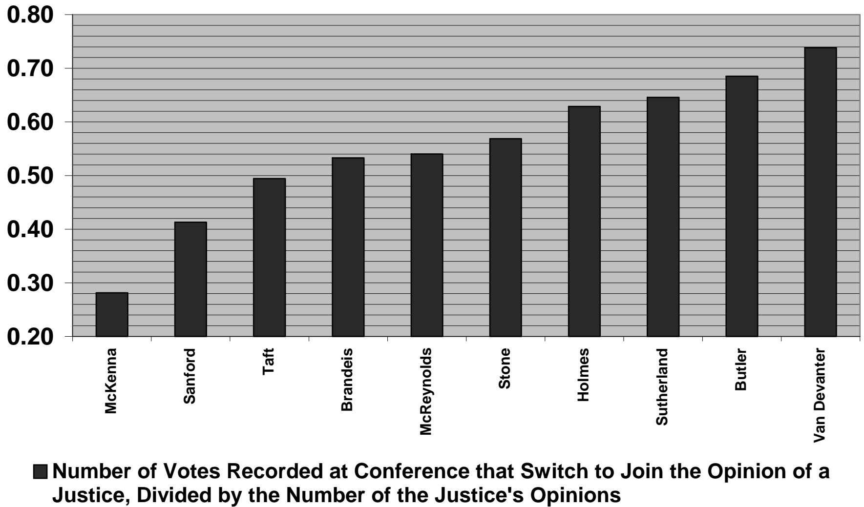
Figure J: The Ability of a Justice to Attract Votes
