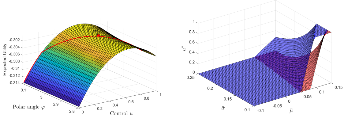
Figure 3: Left: F(u, \varphi) for the static portfolio optimization case study for a fixed \bar{\mu}, \bar{\sigma} . The red line denotes the profile minimizers u \mapsto \check{\varphi}(u) . The red dot denotes the saddle point (u^*, \varphi^*) identified via u^* = \arg \max_{u \in [0, 1]} F(u, \check{\varphi}(u)) . Right: u^* \in [0, 1] as a function of \bar{\mu}, \bar{\sigma} for two different robustness levels \kappa = 4.61 (red), \kappa = 1.39 (blue) and k_0 = 10 .
