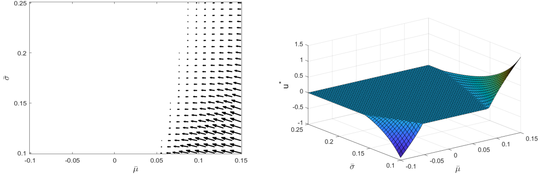
Figure 4: Left panel: quiver plot showing the relative position of (\tilde{\mu}, \tilde{\sigma}) relative to (\bar{\mu}, \bar{\sigma}) . The angle of the quivers is the robustified belief angle \varphi^* and the length is proportional to u^* ; no quiver is shown when u^* = 0 . Right: optimal investment fraction u^* as a function of \bar{\mu}, \bar{\sigma} using unconstrained optimization over \mathbb{R} .
