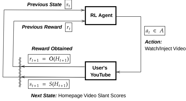
FIGURE 5.1. The proposed RL based approach.
