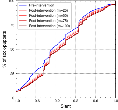
(a) CDFs for left-leaning model.
