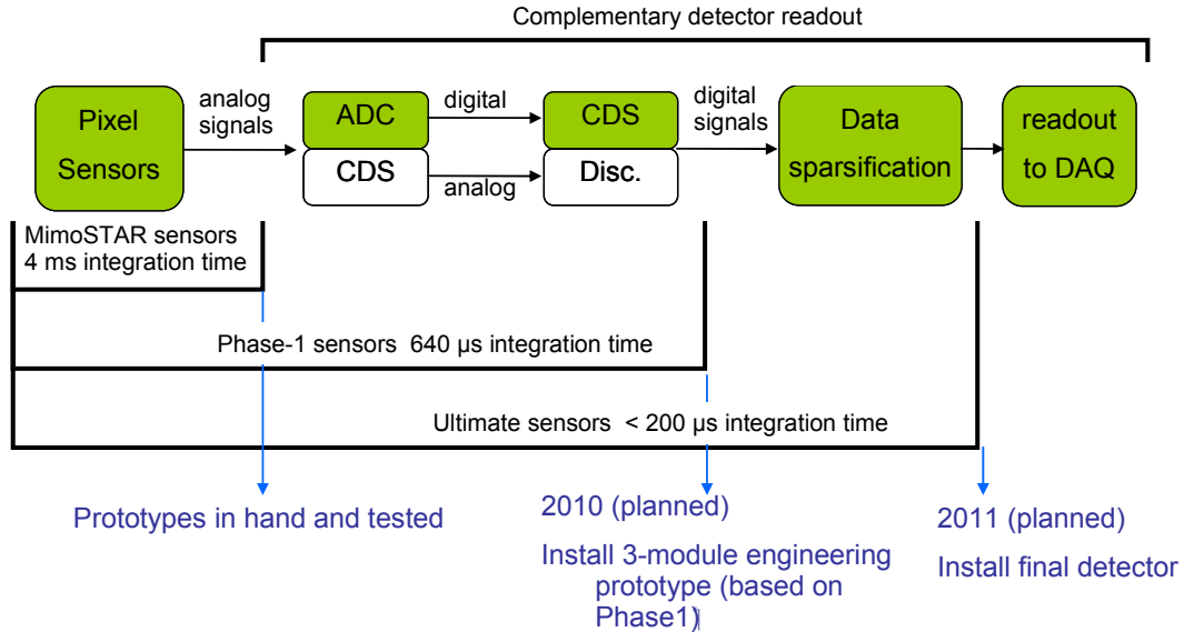
Figure 3 Sensor generation and attendant readout requirements for the STAR Pixel detector.
