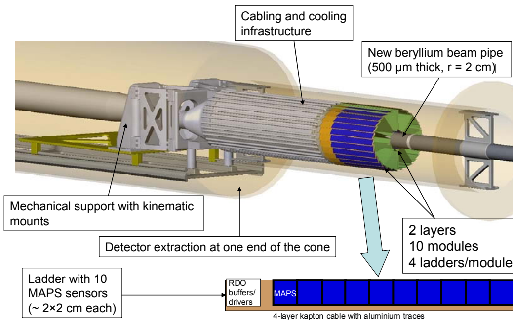
Figure 1 CAD model showing the STAR Pixel detector design. The green trapezoidal support tubes are thin carbon fiber composite. Ten MAPS sensors (shown in blue) are mounted on a readout cable and a carbon fiber carrier plate to form ladder assemblies. Ladder assemblies are placed in overlapping positions with three ladders on the outside and one ladder on the inside of each support tube. There are five support tubes in each half-detector assembly for a total of 40 ladders and 400 2 \times 2 cm. sensors.
