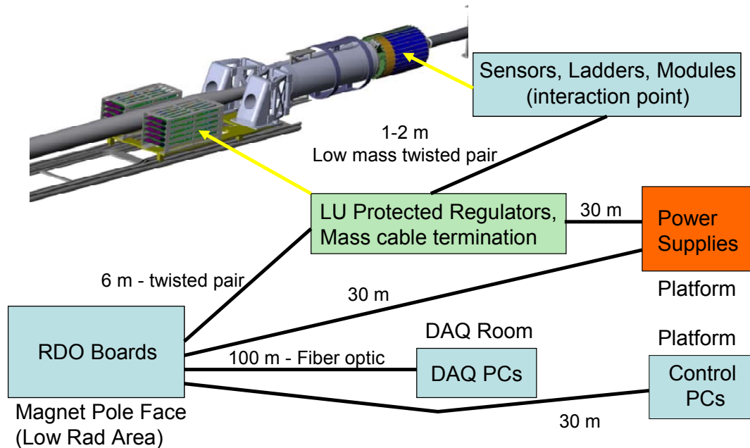
Figure 4 Physical layout of the readout system components for the Pixel detector.
