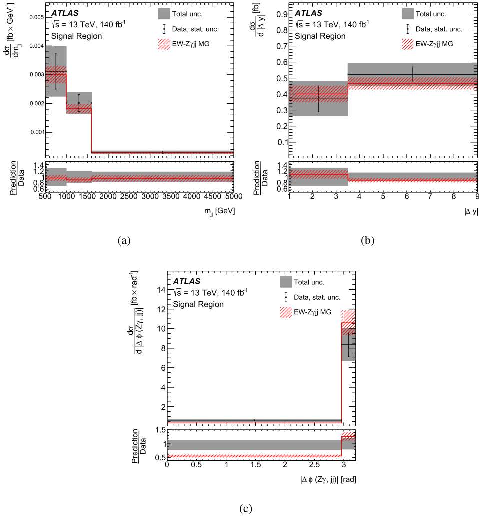
Fig. 4. The EW - Z\gamma jj differential cross-section in the Signal Region as a function of (a) the dijet invariant mass, (b) the dijet rapidity difference and (c) the Z\gamma and dijet azimuthal difference. The lower panels show the ratios of the MC predictions to the data. The band around the unfolded data represents the total uncertainty (including statistical uncertainty) and takes into account the correlations as obtained from the fit. The hatched area represents the uncertainty in the prediction. Events beyond the upper limit of the histogram are included in the last bin.
