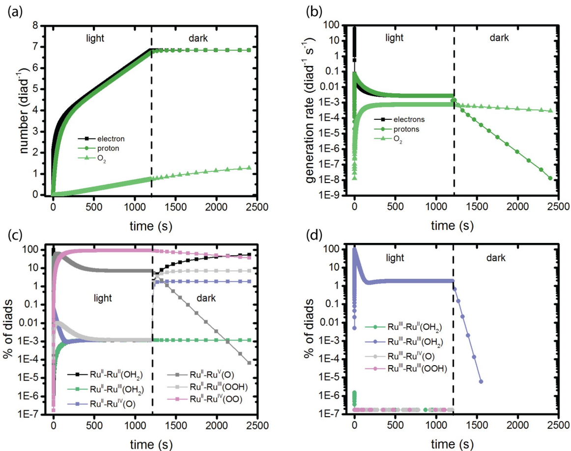
Figure 2. Observables predicted by the simulations in a 1200s light – 1200s dark sequence. (a) total electrons, protons and O 2 generated per diad; (b) rate of electron, proton and O 2 generation per diad per second; (c) diads present with dye in the Ru II state; (d) diads present with the dye in the Ru III state. The populations in panels (c) and (d) together add up to 100%. The colors correspond to the species present in each catalytic stage, Figure 1.
