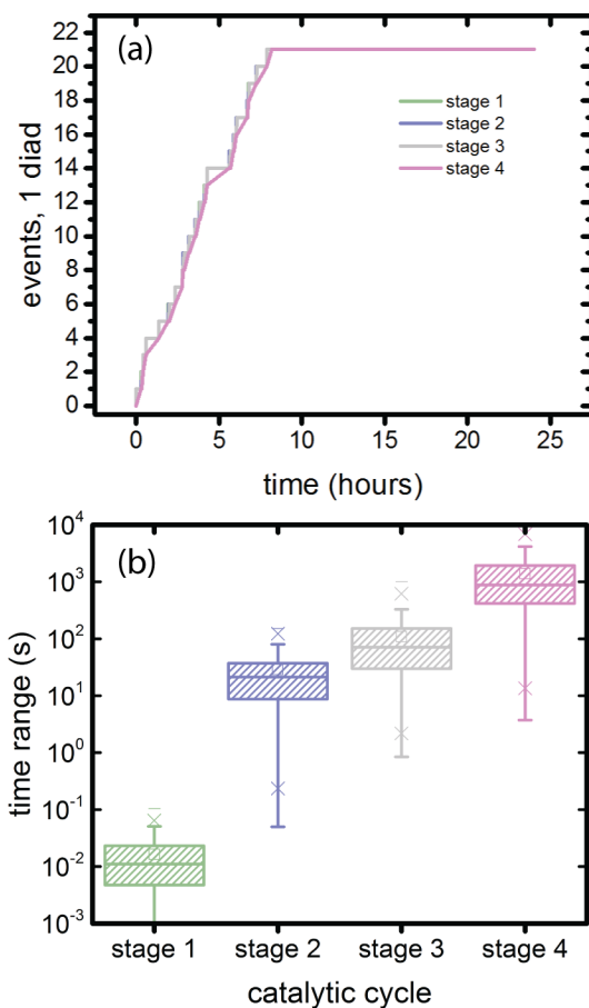
Figure 7. Progression of a single diad through the 4 catalytic stages during 8 hours of illumination followed by 12 hours in the dark. (a) the number of times the diad reaches each stage (typical trace); (b) distribution of times a diad takes to complete each stage (all data).
