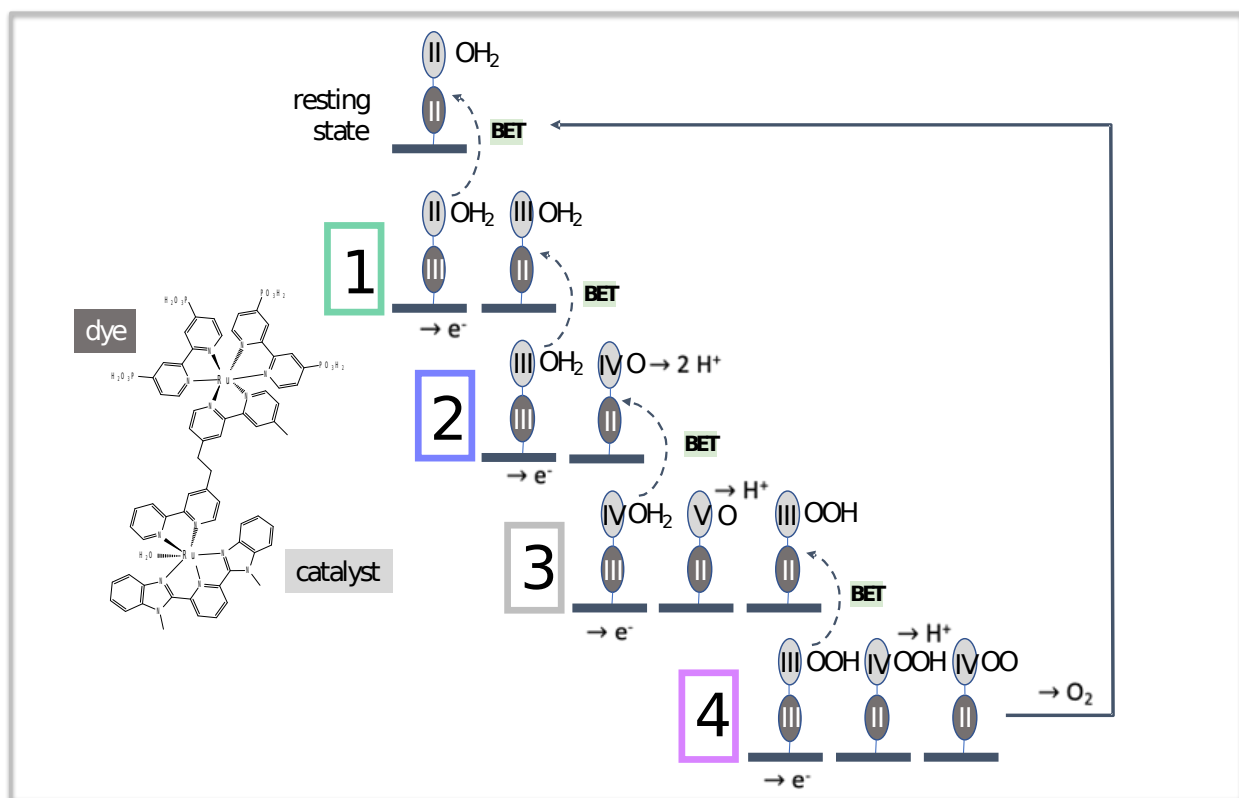
Figure 1. The four stages of water oxidation catalysis driven by photoexcitation of dyes in the Ru II state. A photoexcitation step begins each cycle, oxidizing the dye in the diad product of the preceding step. The color scheme, used throughout this paper, is as follows: dye: dark gray; catalyst: medium gray; resting state of the diad: black; stage 1: gray-green; stage 2: dark lavender; stage 3: light gray; stage 4: rose. The dashed arrows connecting a stage to its preceding one denote back electron transfer processes that reduce the oxidized dye or the oxidized catalyst.
