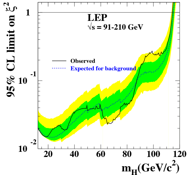
Figure 5: The 95% confidence level upper bound on the ratio \xi^2 = (g_{HZZ}/g_{HZZ}^{\text{SM}})^2 [17]. The solid line indicates the observed limit, and the dashed line indicates the median limit expected in the absence of a Higgs boson signal. The dark and light shaded bands around the expected limit line correspond to the 68% and 95% probability bands, indicating the range of statistical fluctuations of the expected outcomes. The horizontal line corresponds to the Standard Model coupling. Standard Model Higgs boson decay branching fractions are assumed.
