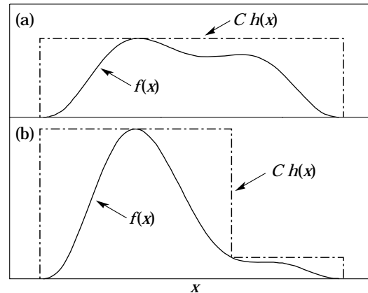
Figure 34.2: Illustration of the acceptance-rejection method. Random points are chosen inside the upper bounding figure, and rejected if the ordinate exceeds f(x) . The lower figure illustrates a method to increase the efficiency (see text).
