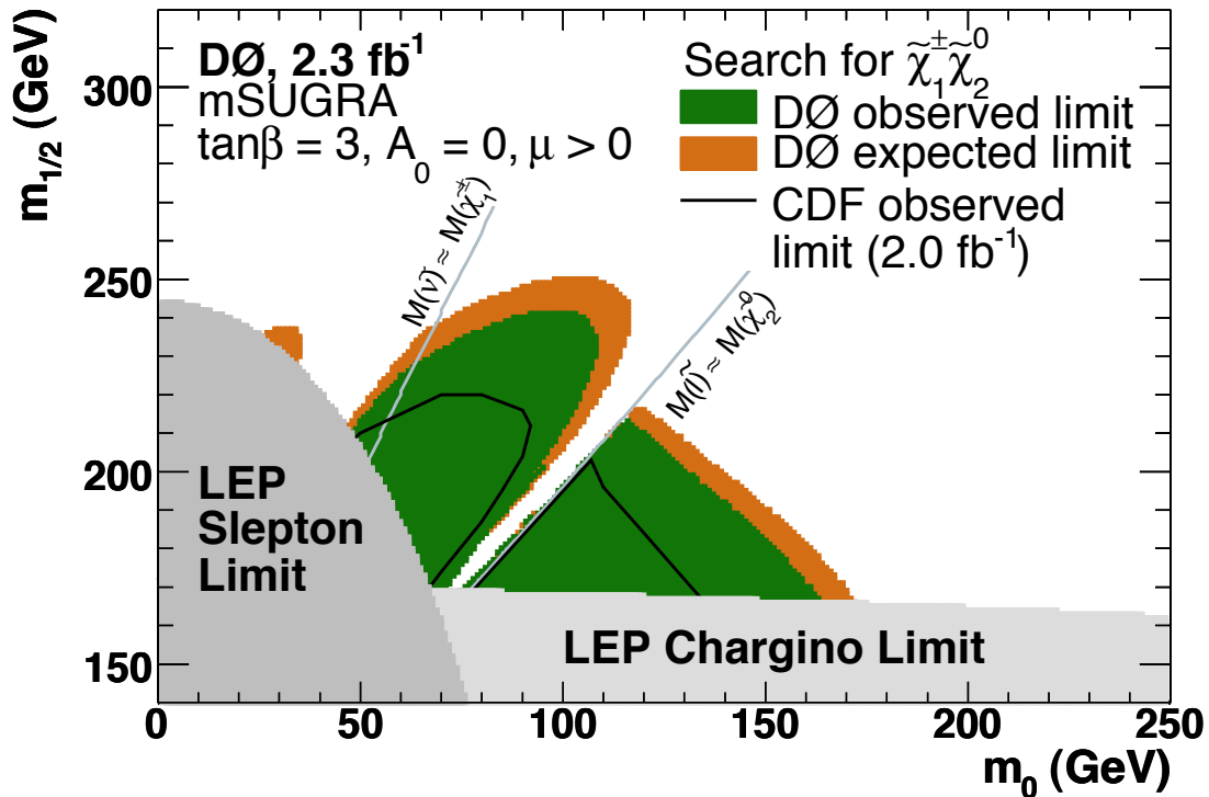
Figure 6: Regions in the (m_0, m_{1/2}) plane excluded by the D\bar{0} search for tripletons and by the LEP experiments.
