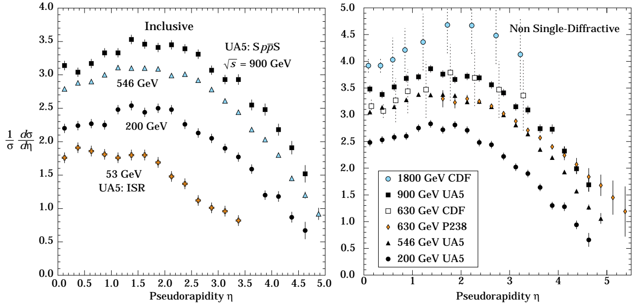
Figure 41.4: Charged particle pseudorapidity distributions in \bar{p}p collisions for 53 \text{ GeV} \leq \sqrt{s} \leq 1800 \text{ GeV} . UA5 data from the S\bar{p}p\bar{S} are taken from G.J. Alner et al. , Z. Phys. C33 , 1 (1986), and from the ISR from K. Alpgöard et al. , Phys. Lett. 112B , 193 (1982). The UA5 data are shown for both the full inelastic cross section and with singly diffractive events excluded. Additional non single-diffractive measurements are available from CDF at the Tevatron, F. Abe et al. , Phys. Rev. D41 , 2330 (1990) and Experiment P238 at the S\bar{p}p\bar{S} , R. Harr et al. , Phys. Lett. B401 , 176 (1997). (Courtesy of D.R. Ward, Cambridge Univ., 1999)
