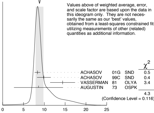
WEIGHTED AVERAGE 8.8±0.9 (Error scaled by 1.5)
