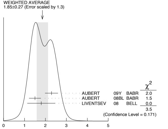
\Gamma(\bar{D}_2^*(2460)^0\ell^+\nu_\ell \times B(\bar{D}_2^0 \rightarrow D^{*+}\pi^-))/\Gamma_{\text{total}} (units 10^{-3} )
