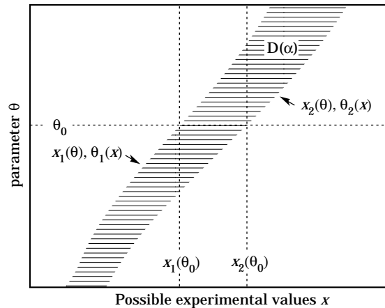
Figure 33.3: Construction of the confidence belt (see text).
