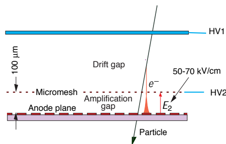
Figure 28.11: Schematic drawing of the Micromegas detector.
