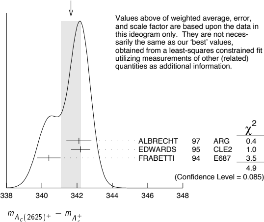
WEIGHTED AVERAGE 341.7 ± 0.6 (Error scaled by 1.6)
