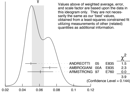
WEIGHTED AVERAGE 0.058±0.007 (Error scaled by 1.4)
