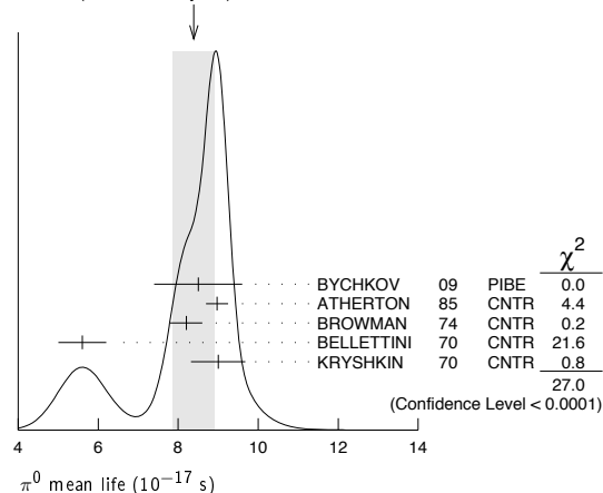
WEIGHTED AVERAGE 8.4 ± 0.5 (Error scaled by 2.6)
