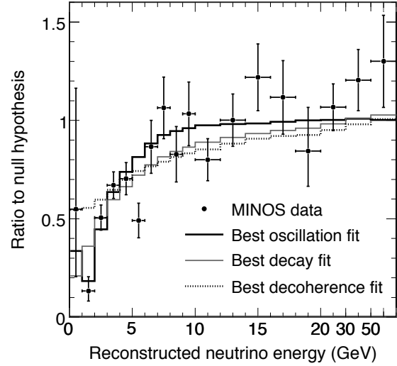
Figure 13.9: Ratio of the MINOS far detector data and the expected spectrum for no oscillations. The best-fit with the hypothesis of \nu_\mu \rightarrow \nu_\tau oscillations as well as the best fit to alternative models (neutrino decay and decoherence) is also shown. This figure is taken from Ref. 22.
