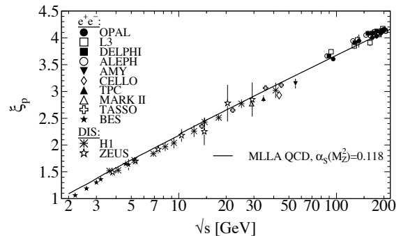
Figure 17.5: Evolution of the peak position, \xi_p , of the \xi distribution with the CM energy \sqrt{s} . The MLLA QCD prediction using \alpha_s(s = M_Z^2) = 0.118 is superimposed to the data of Refs. [25,27,28,31–33,35,40,53,54,69,70,73–81].
