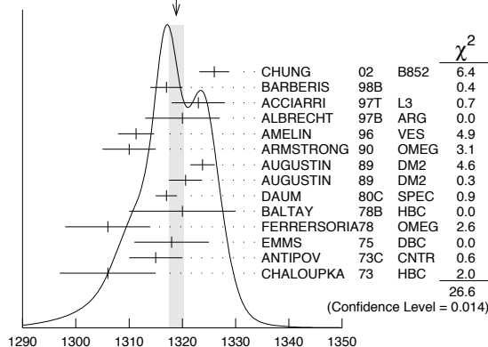
WEIGHTED AVERAGE 1318.9±1.4 (Error scaled by 1.4)
