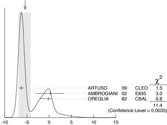
WEIGHTED AVERAGE -5.4 +1.2 -1.5 (Error scaled by 2.4)
