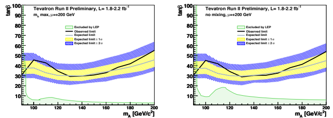
Figure 11: The 95% C.L. MSSM exclusion contours obtained by a combination of the CDF and D\phi searches for H \rightarrow \tau^+\tau^- in the m_h -max (left) and no -mixing (right) benchmark scenarios, both with \mu = 200 GeV, projected onto the (m_A, \tan\beta) plane [147]. The regions above the solid black line are excluded, and the shaded and hatched bands centered on the lighter line show the distributions of expected exclusions in the absence of a signal. Also shown are the regions excluded by LEP searches [18], assuming a top quark mass of 174.3 GeV. The Tevatron results are not sensitive to the precise value of the top quark mass. Color version at end of book.
