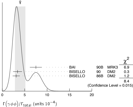
WEIGHTED AVERAGE 4.0 \pm 1.2 (Error scaled by 2.1)
