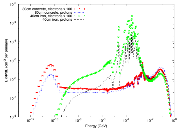
Figure 30.2: Neutron energy spectra calculated with the FLUKA code [6,7] from 25 GeV proton and electron beams on a thick copper target. Spectra are evaluated at 90° to the beam direction behind 80 cm of concrete or 40 cm of iron. All spectra are normalized per beam particle. In addition, spectra for electron beam are multiplied by a factor of 100. See full-color version on color pages at end of book.
