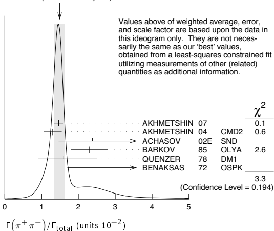
WEIGHTED AVERAGE 1.49 ± 0.13 (Error scaled by 1.3)
