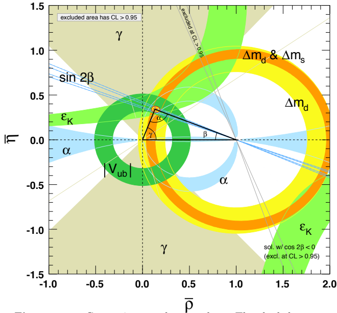
Figure 11.2: Constraints on the \bar{\rho}, \bar{\eta} plane. The shaded areas have 95% CL. Color version at end of book.
