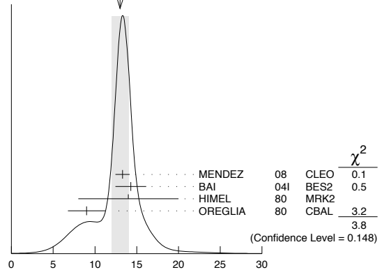
WEIGHTED AVERAGE 13.0±1.0 (Error scaled by 1.4)
