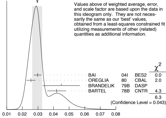
WEIGHTED AVERAGE 0.0296±0.0031 (Error scaled by 1.8)
