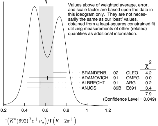
WEIGHTED AVERAGE 0.61 ± 0.07 (Error scaled by 1.6)
