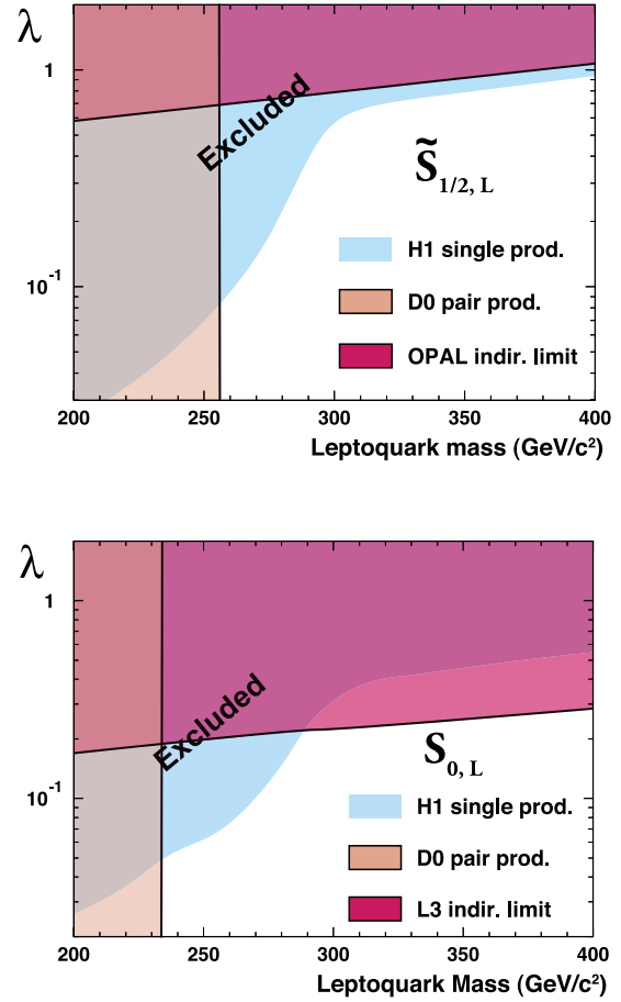
Figure 1: Limits on two typical first-generation scalar leptoquark states in the mass-coupling plane. The upper figure is for a weak-isodoublet, weak-hypercharge 7/6 , 3B + L = 0 leptoquark state, while the lower figure is for a weak-isosinglet, weak-hypercharge -1/3 , 3B + L = 2 state. Color version at end of book.
