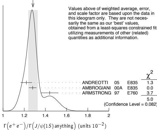
WEIGHTED AVERAGE 1.28±0.04 (Error scaled by 1.6)
