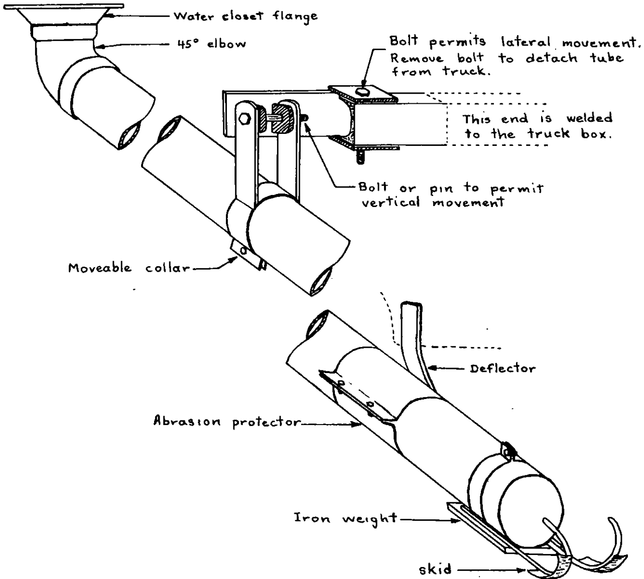
Fig. 1. Design of bait dispenser, made from an 8-foot length of 3-inch-diameter plastic sewer pipe.
