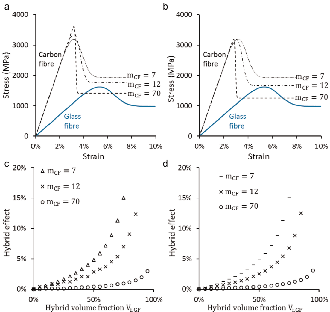
Fig. 7. Stress–strain diagrams for the reference composites with various values of the Weibull modulus, m_{CF} , for (a) the same composite failure strain, and (b) the same composite strength. The hybrid effect is plotted as a function of the hybrid volume fraction for (c) the same reference composite failure strain, and (d) the same reference composite strength.
