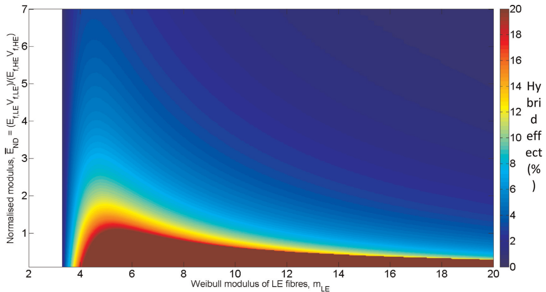
Fig. 6. Contour plot for the hybrid effect as a function of the Weibull modulus of the LE fibre and the normalised modulus, without the linear elastic assumption for the HE fibres. Values above 20% are topped off. (For interpretation of the references to color in this figure, the reader is referred to the web version of this article.)
