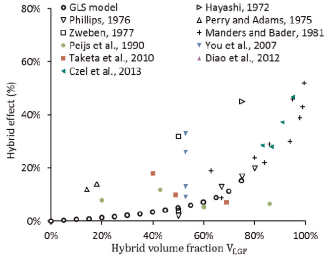
Fig. 3. Comparison of the hybrid effect predicted by GLS with experimental data available in literature.
