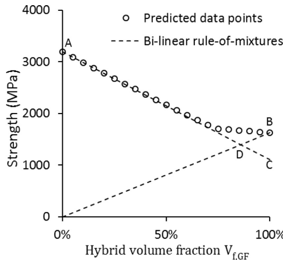
Fig. 4. The hybrid effect for strength, compared with the bi-linear rule-of-mixtures.
