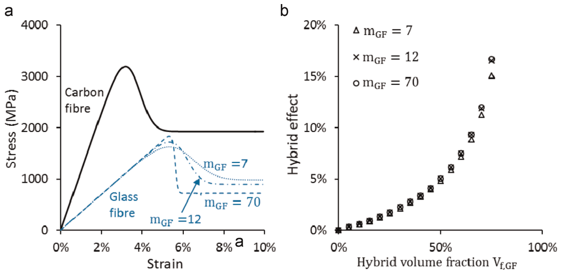
Fig. 8. (a) Stress–strain diagram of the glass fibre reference composite with various values of the glass fibre Weibull modulus, m_{GF} , when the composite failure strain is held fixed and (b) its influence on the hybrid effect.
