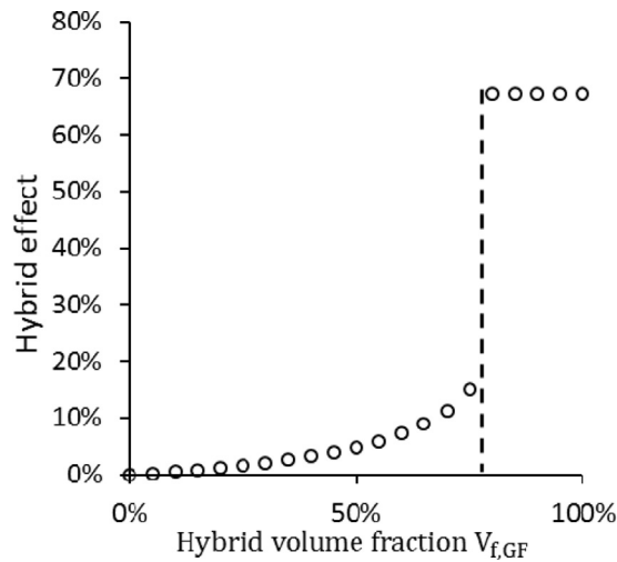
Fig. 2. The hybrid effect as a function of the hybrid volume fraction. The dashed line represents the hybrid volume fraction beyond which the failure strain is controlled entirely by that of the glass fibres.
