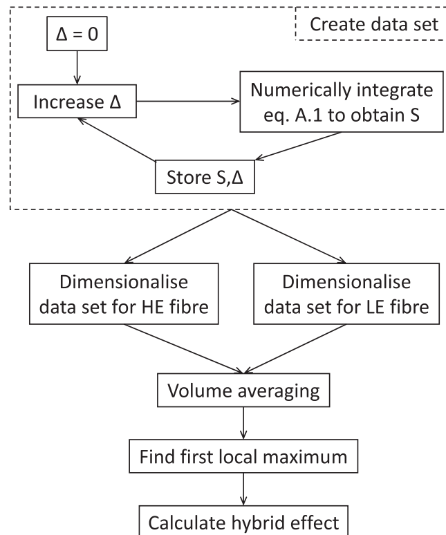
Fig. A.1. Flow chart of the GLS model for hybrid composites.
