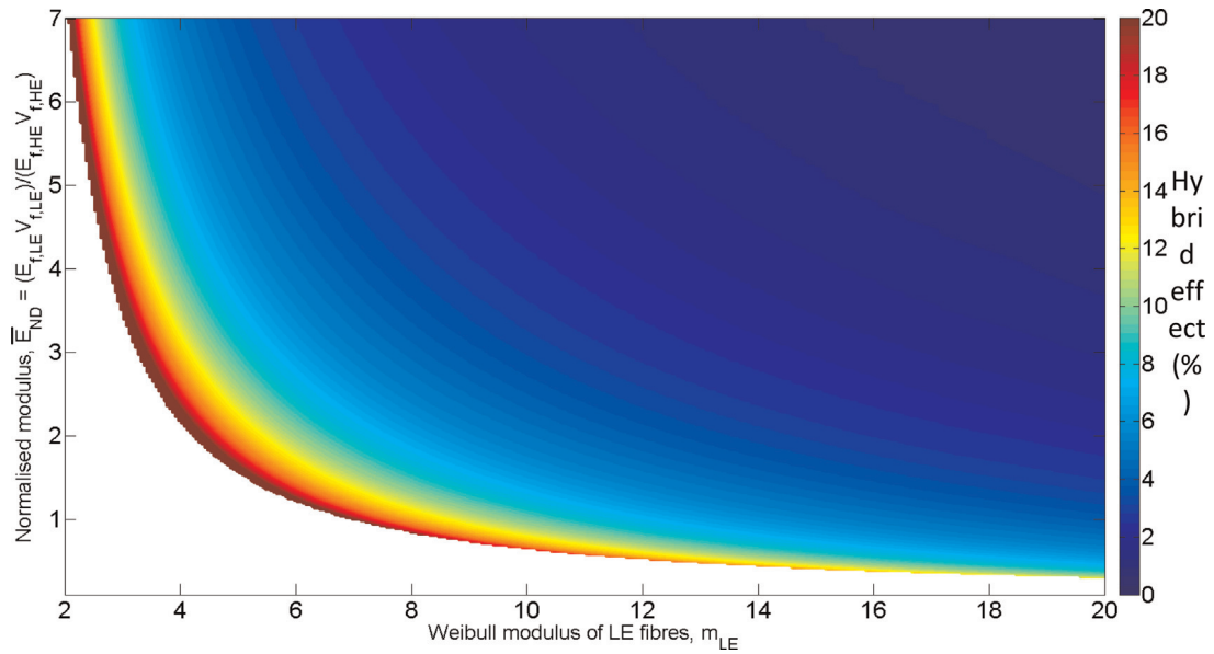
Fig. 5. Contour plot for the hybrid effect as a function of the Weibull modulus of the LE fibre and the normalised modulus, under the assumption that the HE fibres remain linear elastic. Values above 20% are topped off.
