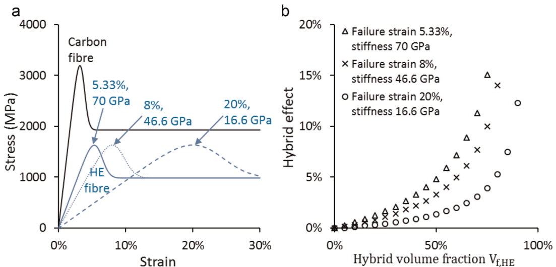
Fig. 9. (a) Stress–strain diagrams for a HE fibre composites with various HE failure strains and fibre stiffnesses, but the same tensile strength, and (b) its influence on the hybrid effect.
