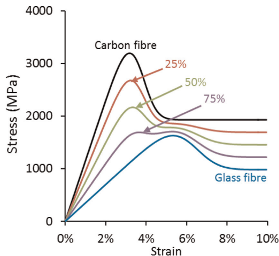
Fig. 1. Predicted stress–strain curves of the two reference composites and three hybrid composites, with their hybrid volume fractions, V_{f,GF} , indicated.
