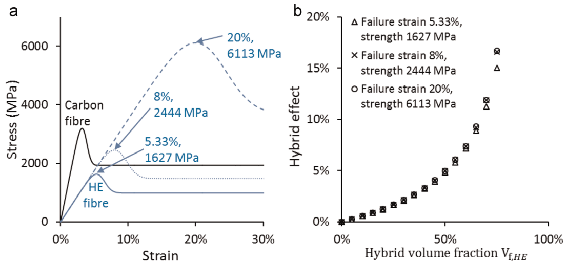
Fig. 10. (a) Stress–strain diagrams for a HE fibre composites with various HE failure strains and strengths but the same fibre tensile modulus, and (b) its influence on the hybrid effect.
