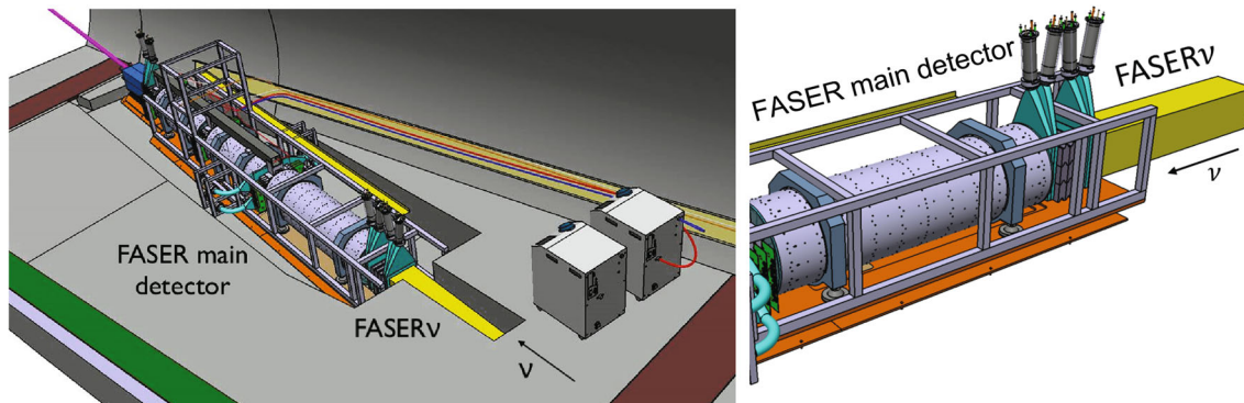
Fig. 2 View of FASER, including the FASER \nu detector, in tunnel TI12, 480 m downstream from the ATLAS IP along the beam collision axis. The FASER \nu detector is a 25 cm \times 25 cm \times 1.35 m emulsion detector, consisting of 1000 layers of emulsion films interleaved with
