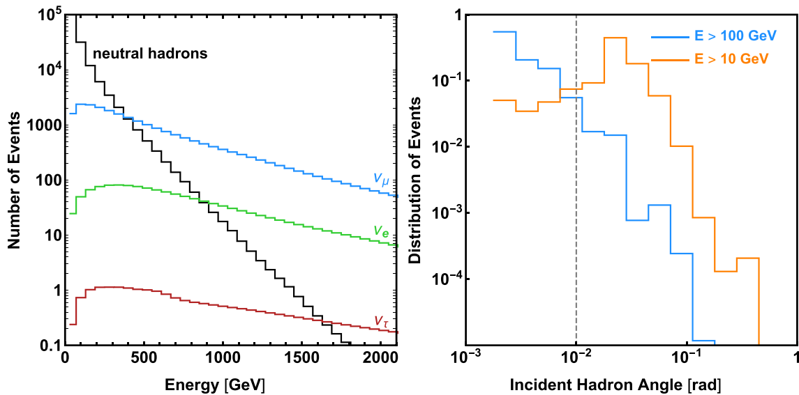
Fig. 15 The energy and angular distributions of neutral hadrons that are produced by negative muon interactions and pass through \text{FASER}\nu in Run 3. Left : The energy spectrum of neutral hadrons produced in the rock in front of \text{FASER}\nu and produced within the detector (black) as well as neutrinos interacting with the detector for an integrated luminosity of 150 \text{ fb}^{-1} : \nu_e (red), \nu_\mu (blue) and \nu_\tau (green). Right : The angular
