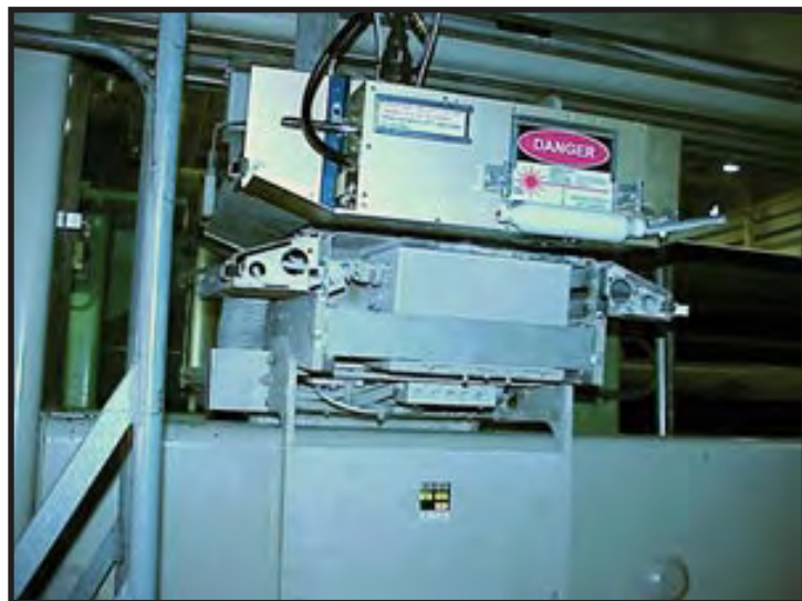
Figure 1. The laser ultrasonic sensor was successfully tested at a working paper mill.
