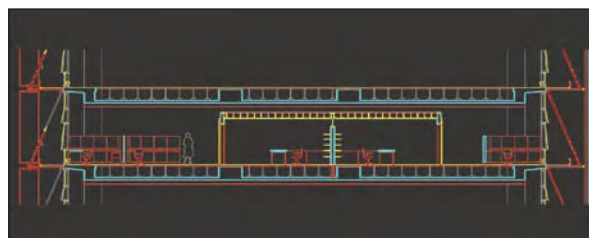
Figure 1. A cross-section of the building, in which air flows through windows that can be opened.
