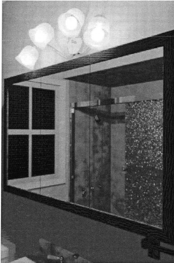
Figure 9. Naive histogram equalization allows us to see the area around the light sources but contrast is exaggerated in other areas such as the shower tiles.
