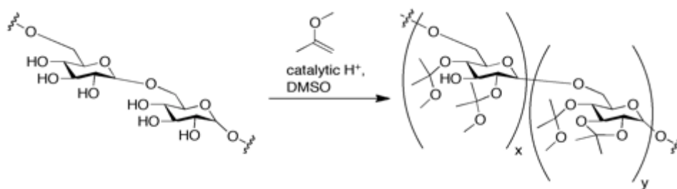
Scheme 3.1. Synthesis of acetalated dextran (AcDex)
