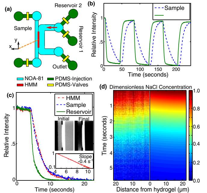
FIG. 5. (a) Device geometry for prompt reservoir solution swapping using PDMS valves and rapid dialysis in the sample channel using an HMM. Panel (b) and Video 4: Swapping between 250-mM-NaCl (bright) and 0-mM-NaCl (dark) solutions in a 150- \mu\text{m} -wide sample channel, with a fluorescent NaCl indicator. (c) Swapping time is greatly decreased by decreasing sample-channel width (here, 23 \mu\text{m} wide). Inset graph: Semilog plot of HMM intensity shows exponential decay of salt concentration in HMM. Panel (d) and Video 5: Observed dynamics of NaCl concentration along the x axis of the sample channel are well predicted by the one-dimensional diffusion equation.
