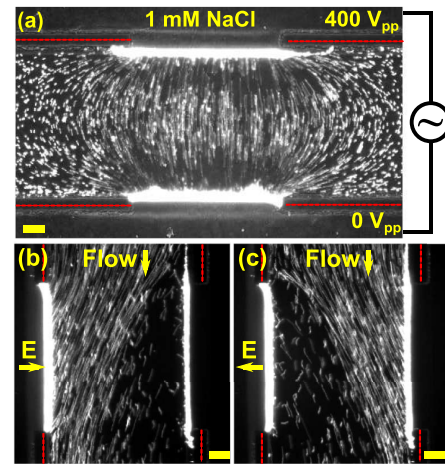
FIG. 6. (a) An ac potential applied between reservoir channel inlets drives an electric field that only crosses the sample channel through the HMMs. Fluorescent colloids in the sample channel oscillate electrophoretically, tracing local electric-field lines much like iron filings align with magnetic fields. Panels (b-c) and Video 6: Continuous-flow electrophoretic separations of negatively charged colloids by applying a dc electric field E transverse to the flow. Scale bars: 20 \mu\text{m} .
