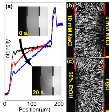
FIG. 7. Concentration gradients created locally within microchannels. (a) Direct gradient visualization with Oregon Green fluorescent dye at 0 (black), 10 (red), and 20 (blue) seconds after stopping flow. Panel (b) and Video 7: Diffusiophoretic motion of fluorescent colloids up a NaCl gradient. Panel (c) and Video 8: Solvophoretic motion down an ethanol gradient. Scale bar: 20 \mu\text{m} .
