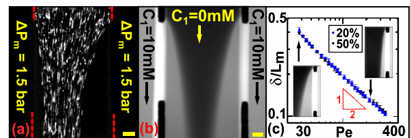
FIG. 4. (a) In the three-channel device [Figs. 1(b), 1(c), and 2], the amount of convection admitted by HMMs at large transmembrane pressure drops, here \Delta P_m = 1.5 bar, is lower for a highly cross-linked HMM (50% v/v, left) than for a lightly cross-linked HMM (20%, right). Tracer particles are focused towards the center of the channel by transmembrane flow from the side channels. (b) The diffusive flux through a lightly cross-linked membrane (20% v/v, right) is nearly identical to that through a highly cross-linked (50% v/v, left) membrane. (c) After diffusing through each HMM, the pH buffer is convected downstream, forming a boundary layer whose thickness decreases with Peclet number (flow velocity) like \text{Pe}^{1/2} , as expected for 2D convection-diffusion. Scale bars: 20 \mu\text{m} .
