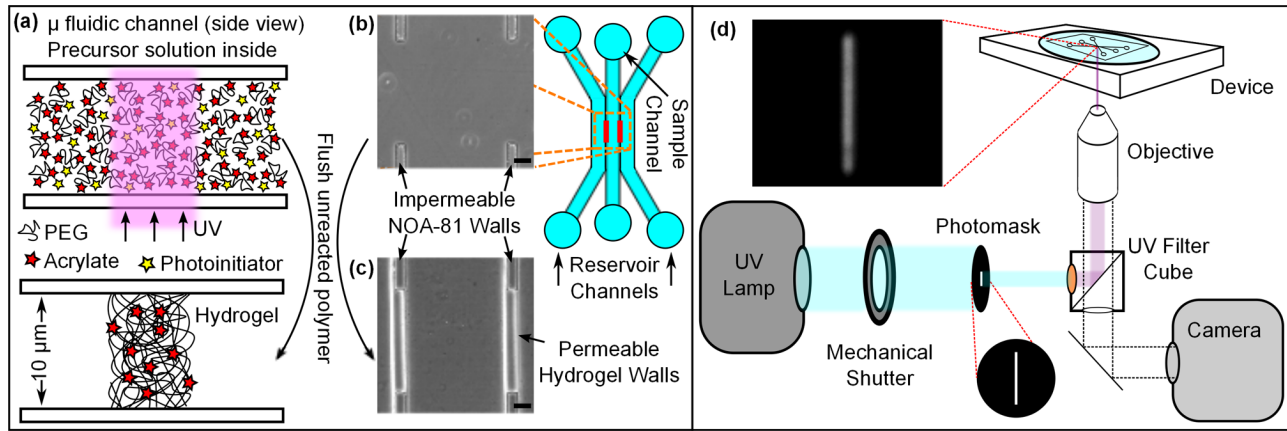
FIG. 1. Fabrication of HMMs. (a) A UV-polymerizable solution of poly(ethylene-glycol)-diacrylate and photoinitiator initially fills a three-channel microfluidic device (b), with gaps in the walls between channels. Patterned UV light is used to cross-link the hydrogel in two specified rectangular regions (width: 10–20 \mu\text{m} ) filling the gaps in the walls. (c) After flushing the unreacted solution, hydrogel microwindow membranes remain (phase contrast, scale bar = 20 \mu\text{m} ). (d) Simplified microscope schematic for fabricating HMMs. The microfluidic device is placed on the microscope stage, and a photomask is inserted into the microscope field aperture. A computer-controlled mechanical shutter exposes the PEG-DA solution to UV irradiation for the desired exposure time. Inset: Natural fluorescence of NOA-81 optical glue enables the patterned UV light to be aligned.
