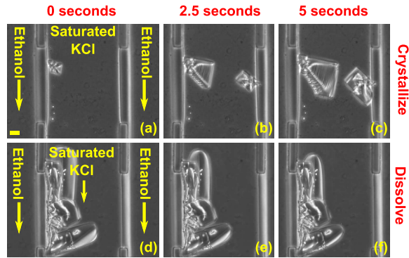
FIG. 3. Antisolvent diffuses from the reservoir channels across HMMs into a saturated aqueous salt solution in the sample channel, depicted in the three-channel device of Figs. 1(b) and 1(c). (a-c) Upon stopping KCl flow in the sample channel, ethanol diffuses through the HMMs. As ethanol concentration progressively increases near the HMM, KCl solubility decreases, triggering nucleation and growth of KCl crystals. (d-f) Resuming convective delivery of fresh aqueous KCl solution flushes away the ethanol, restoring KCl solubility to its bulk aqueous value, and dissolving the crystals. (See Videos 2 and 3.) (Phase contrast, scale bar = 20 \mu\text{m} .)
