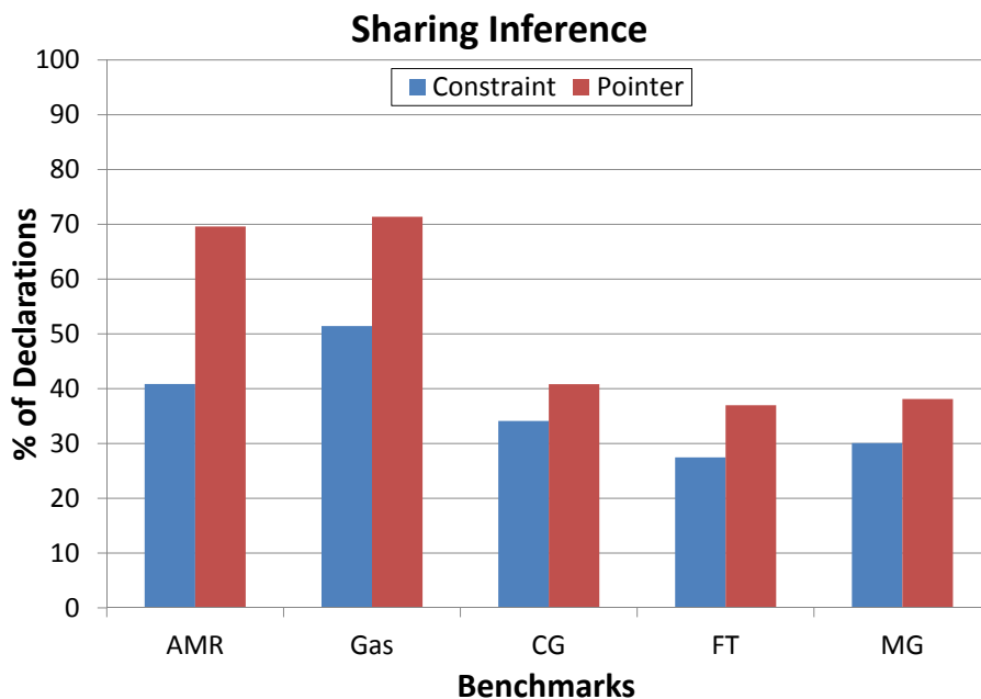
Figure 8.35: Sharing inference results for some Titanium programs.
