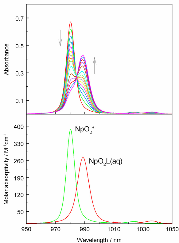
Fig. 2 Spectrophotometric titrations of Np(V)/DMOGA complex ( I = 1.0 \text{ mol}\cdot\text{dm}^{-3} , t = 25^\circ\text{C} ), (top) normalized absorption spectra, (bottom) molar absorptivities. V^0 = 2.50 \text{ mL} , C_{\text{Np}^0}/C_{\text{H}^0} = 1.74/0.0006 \text{ mmol}\cdot\text{dm}^{-3} ; DMOGA titrant: C_{\text{I}}/C_{\text{H}} = 0.0346/0.0148 \text{ mol}\cdot\text{dm}^{-3} , 0.300 \text{ mL} total volume added.
