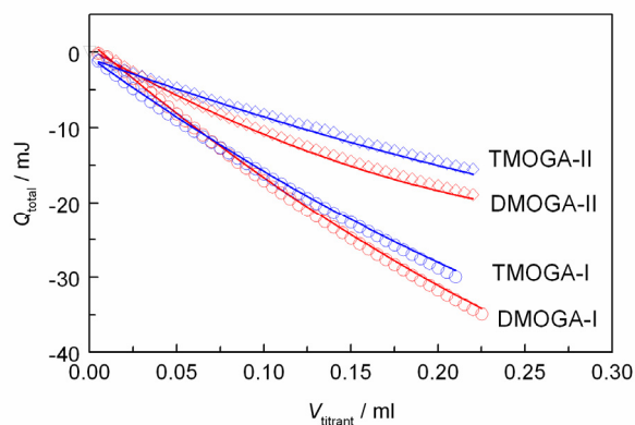
Fig. 3 Calorimetric titrations of Np(V)/DMOGA and Np(V)/TMOGA complexation ( I = 1.0 \text{ mol}\cdot\text{dm}^{-3} , t = 25^\circ\text{C} ), (top) an example thermogram, (bottom) experimental heat (O) and fit (—). V^0 = 0.900 \text{ mL} , C_{\text{Np}^0}/C_{\text{H}^0} = 1.74/0.0006 (I) and 1.16/0.0004 (II) \text{mmol}\cdot\text{dm}^{-3} ; titrant: C_{\text{DMOGA}}/C_{\text{H}} = 0.0570/0.00273 \text{ mol}\cdot\text{dm}^{-3} , C_{\text{TMOGA}} = 0.400 \text{ mol}\cdot\text{dm}^{-3} , about 0.225 \text{ mL} total volume added.
