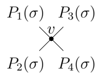
Figure 2.2: The neighborhood of the unique vertex v in G_\sigma satisfying \text{val}(v) + |m^{-1}(v)| = 4 for a codimension-1 cone \sigma in M_{0,n}^{\text{trop}} . Here we visualise m_\sigma^{-1}(v) as half-edges.
