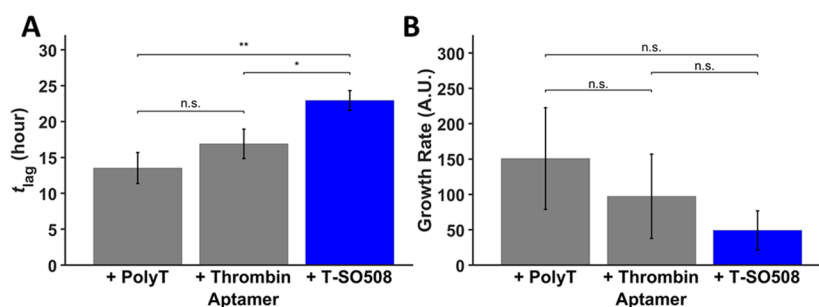
Figure 3. Comparison of effects of the T-SO508 aptamer and control DNA sequences. Samples contained 140 \mu\text{M} \alpha -synuclein, 60 \mu\text{M} ThT, and 10 \mu\text{M} of one of the following: poly-T sequence, thrombin aptamer, or T-SO508. Fluorescence traces were analyzed by MI analysis. (A) T-SO508 prolonged t_{lag} significantly compared to control sequences. (B) In contrast, the growth rate shows no significant difference between T-SO508 and control sequences. Error bars represent one standard error ( n = 6 ; two-sample t test: n.s. = not significant; * indicates p < 0.05 ; ** indicates p < 0.01 ).
