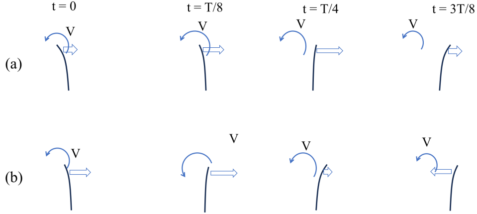
FIG. 10. Schematic illustrations of plate deformation and vortex generation at (a) \kappa = 2 (the case shown in Fig. 9b) and (b) \kappa = 3 (the case shown in Fig. 9c). The arrows indicate the direction and (qualitatively) the speed of horizontal motion at the top end.
