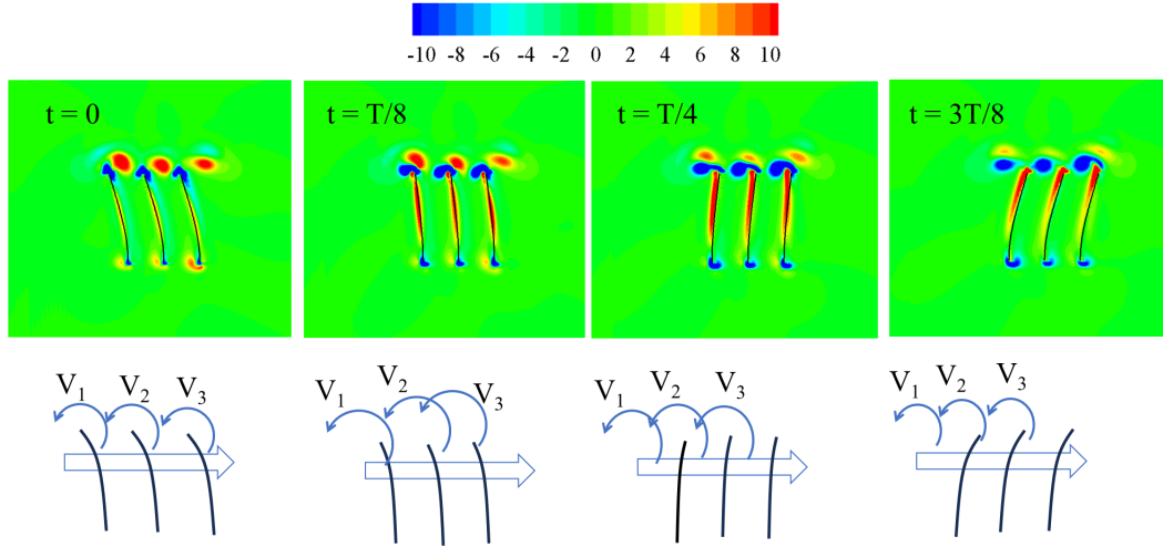
FIG. 11. (Upper row) Snapshots of the flow field around a formation of three plates visualized through vorticity contour during half a period for \kappa = 2 , K_C = 0.5 , and D = 0.4 . (Lower row) Schematic illustrations of the plate deformation and vortex generation. The arrows indicate the direction of horizontal motion at the top ends.
