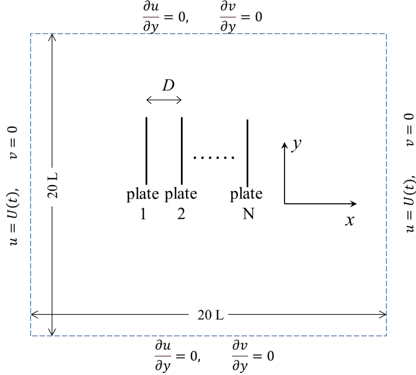
FIG. 1. The computational domain and the boundary conditions.
