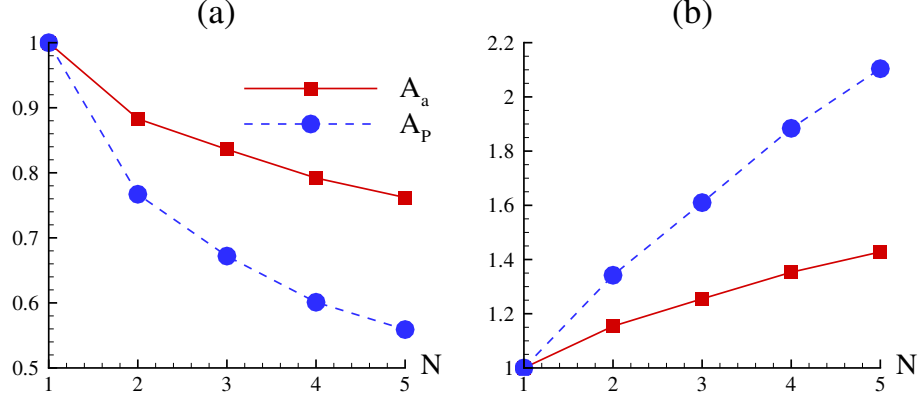
FIG. 5. Amplification factors A_a and A_p at different array size N . (a) \kappa = 1 , K_C = 1 ; (b) \kappa = 2 and K_C = 0.5 . D = 0.2 .
