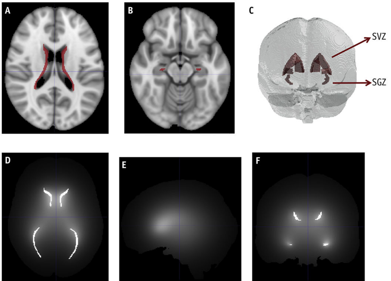
Fig. 1. Two brainstem cell zones, showing the (A) subventricular zone, and (B) subgranular zone, as well as a (C) 3-dimensional rendering of segmented bilateral subventricular and subgranular zones, and (D) axial, (E) sagittal, and (F) coronal views of the proximity map with intensities illustrating the degree of proximity to all stem cell niches. All images are visualized in ITK-SNAP ( www.itksnap.org ).
