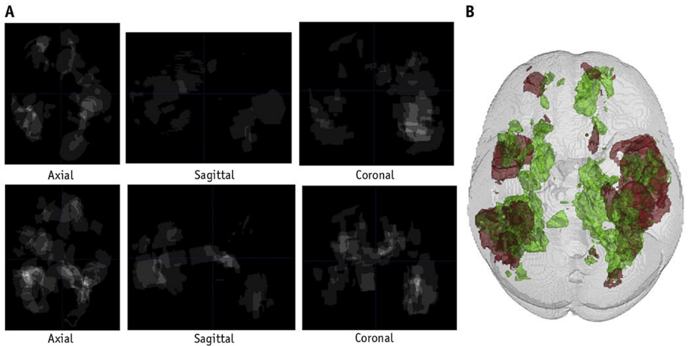
Fig. 3. Overlaid primary and recurrent tumor locations from all subjects, showing (A) axial, sagittal, and coronal views for primary (upper row) and recurrent (bottom row) tumors, and (B) 3-dimensional rendering of primary (red) and recurrent (green) tumors. Primary and recurrent tumors show significant differences in proximity to stem cell niches (medial and center located), using 3 centroid/mean proximity score-based metrics. (A color version of this figure is available at https://doi.org/10.1016/j.ijrobp.2021.02.020 .)
