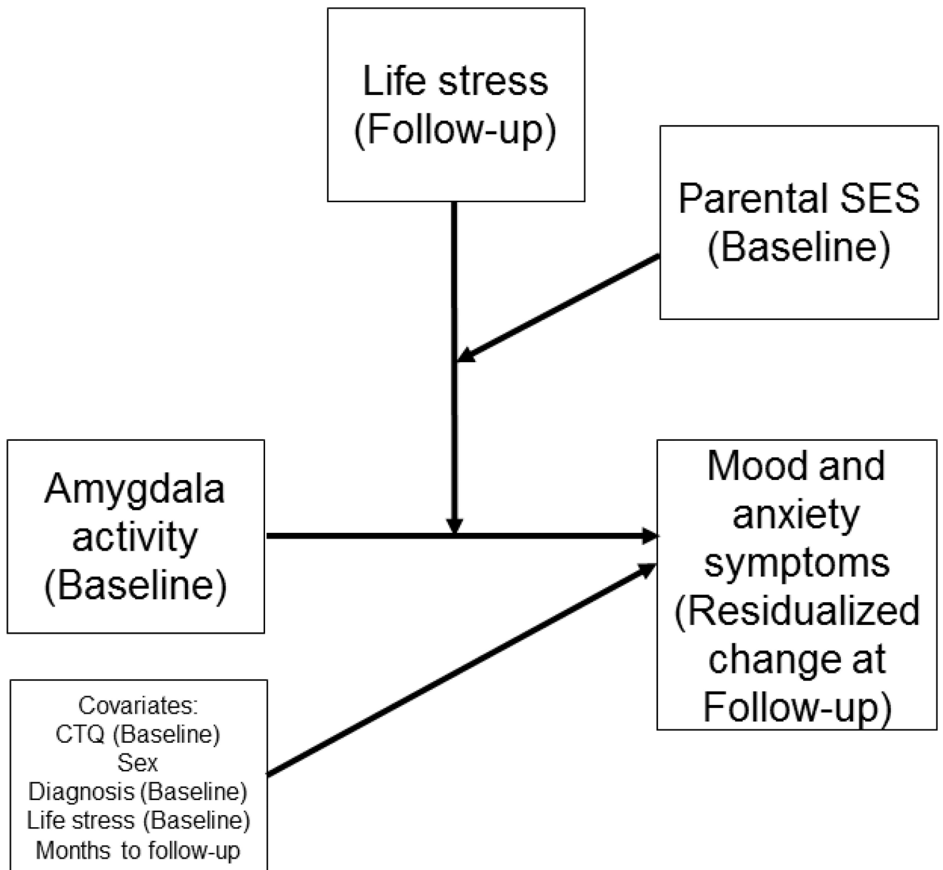
Figure 1. Statistical model
