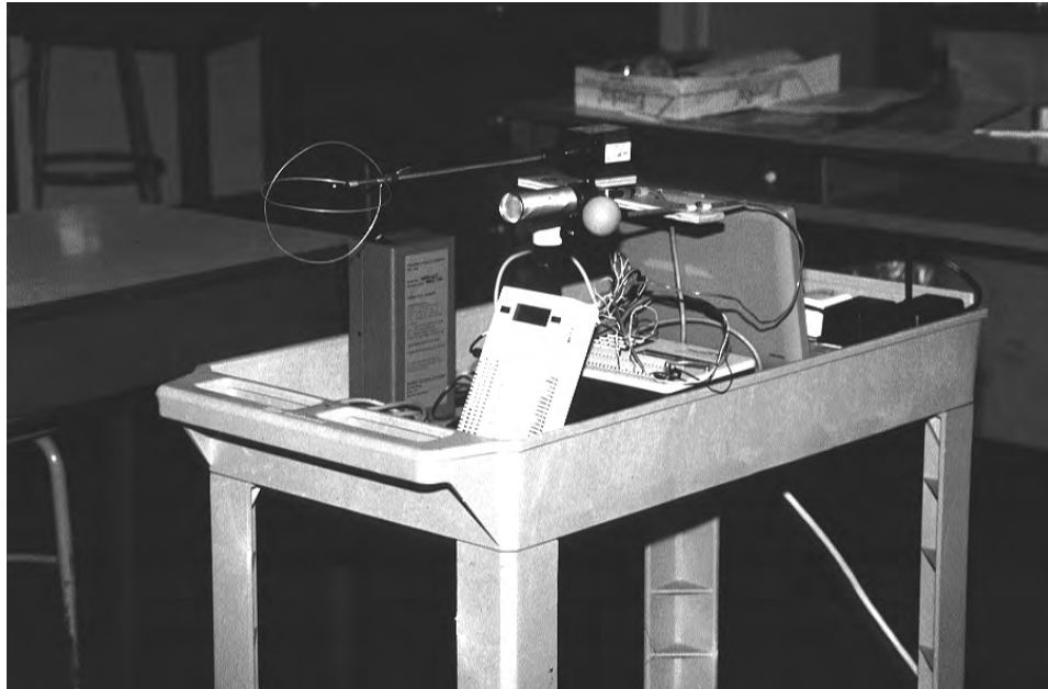
Figure 4.2 Equipment to measure indoor climate
