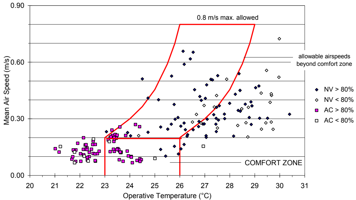
Figure 5.16 Direct thermal acceptability compared to air movement criteria of Standard 55 summer comfort zone (each symbol represents an average of acceptable votes for a classroom visit)
