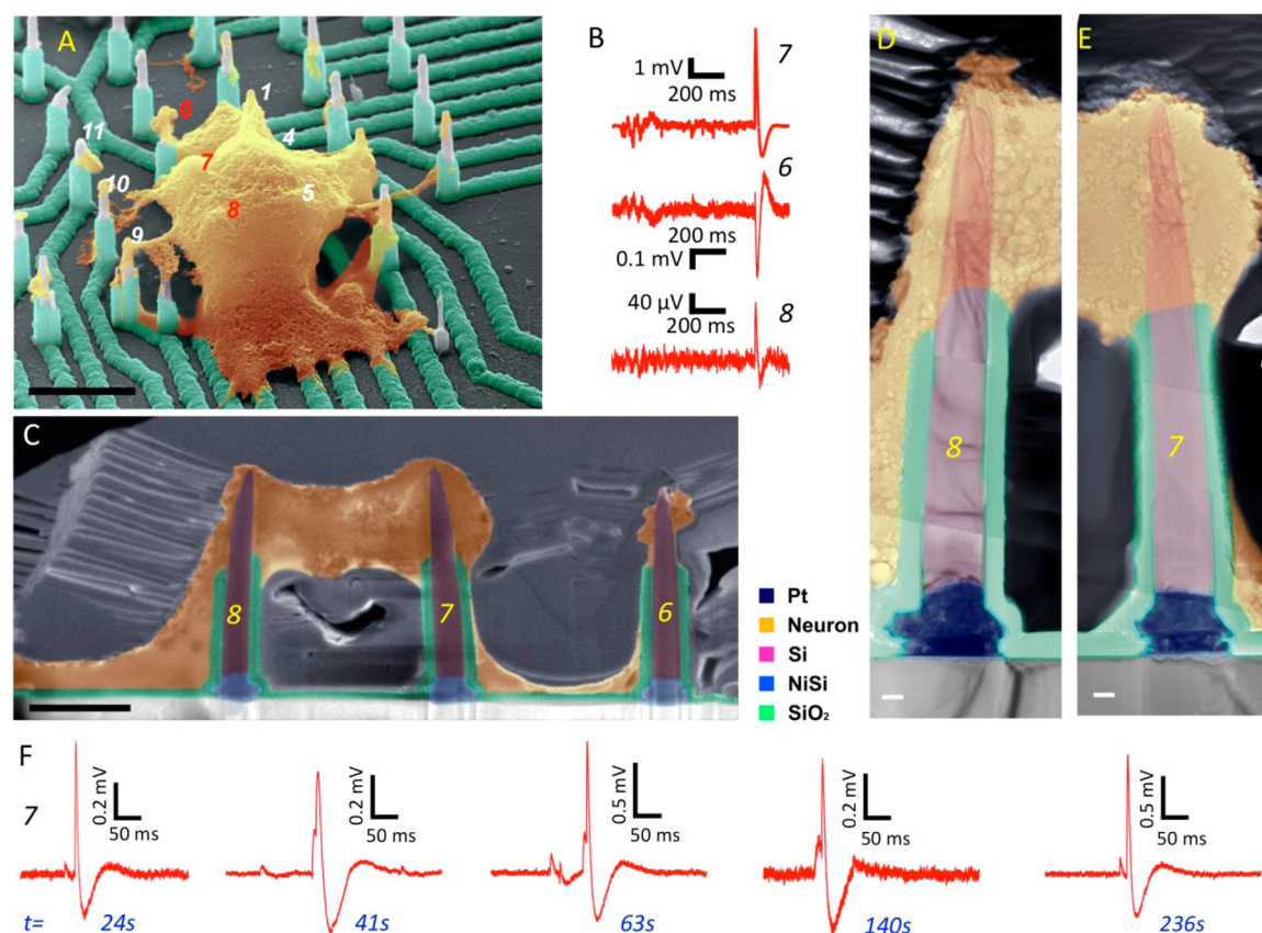
Figure 4. Recording from hiPSC-derived cortical neurons. (A) Colorized angle-view SEM image showing cell morphology and neurite outgrowth to nearby nanowires. Scale bar is 4 \mu\text{m} . (B) Measured potentials on channels 6–8 showing positive potentials for wires 7 and 8 inside the cell and negative potential for wire 6 outside the cell. (C) Colorized SEM image of the Pt coated and FIB thinned cross-section of the cell in panel B. The image shows the cell (yellow colored) engulfing the tops of nanowires 7 and 8, and portions of cell membrane around nanowire 6. Scale bar is 2 \mu\text{m} . Electrophysiology was performed 6 weeks post in vitro culture. (D, E) Higher magnification colorized TEM images collected and stacked to provide a higher resolution close-up to the nanowire-cell interface. The slight bending of the nanowires is likely to have happened during neuron dehydration in preparation for SEM imaging (section 5 of Supporting Information ). Scale bars are 200 nm. (F) Recordings on nanowire number 7 illustrating consistent oscillations prior to action potential firing at different recording times.
