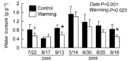
Fig. 1 Soil water content in warmed and control plots during the 2005–2006 growing seasons ( n = 5 ). Bars show mean and SE on each date. Significant effects from repeated-measures ANOVA are shown in italicized text. † P < 0.10 , * P < 0.05 for warming effect within date.
