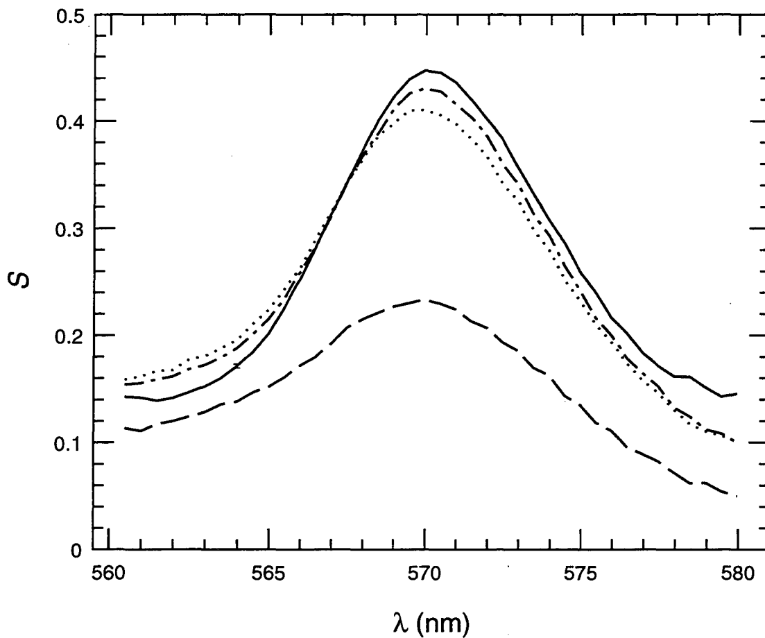
Figure 5.4: Spectra for the \text{PuO}_2^+ \cdot \text{UO}_2^{2+} complex experiment at \mu = 6 \text{ M} . The spectra shown are for a calculated \text{PuO}_2^+ concentration of 0.0924 \text{ mM} (solid line), solution D-1 (dashed line), solution D-2 (dotted line), and solution D-3 (dot-dashed line). See Table 5.4 for the composition of solutions D-1, D-2, and D-3. Spectra are normalized at 567.5 \text{ nm} , the isosbestic point. The error bar at 567.5 \text{ nm} on the solid line is typical of the errors for these spectra.
