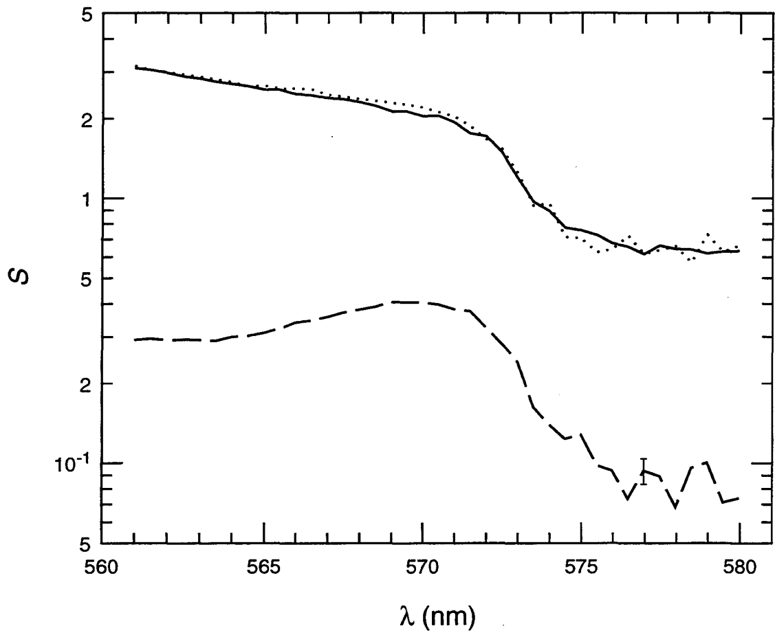
Figure 5.6: Spectra for the \text{PuO}_2^+ \cdot \text{Fe}^{3+} experiment at \mu = 6 M. The spectra shown are for solution Pu-11 (dashed line), solution Fe-2 (solid line), and solution G-2 (dotted line). See Table 5.6 for the composition of the solutions. Spectra have not been normalized. The error bar at 577.0 nm on the dashed line is typical of the error for these spectra above about 574 nm; the error bars below about 574 nm are about the width of the line.
