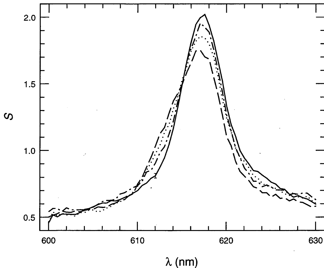
Figure 5.3: Spectra for the \text{NpO}_2^+ \cdot \text{Th}^{4+} complex experiment at \mu = 6 M. The spectra shown are for a calculated \text{NpO}_2^+ concentration of 0.297 mM (solid line), solution C-1 (dashed line), solution C-2 (dotted line), and solution C-3 (dot-dashed line). See Table 5.3 for the compositions of C-1, C-2, and C-3. The spectra did not require any normalization. The error bar at 612.0 nm on the solid line is typical for these spectra. Note the ordinate scale does not begin with 0.
