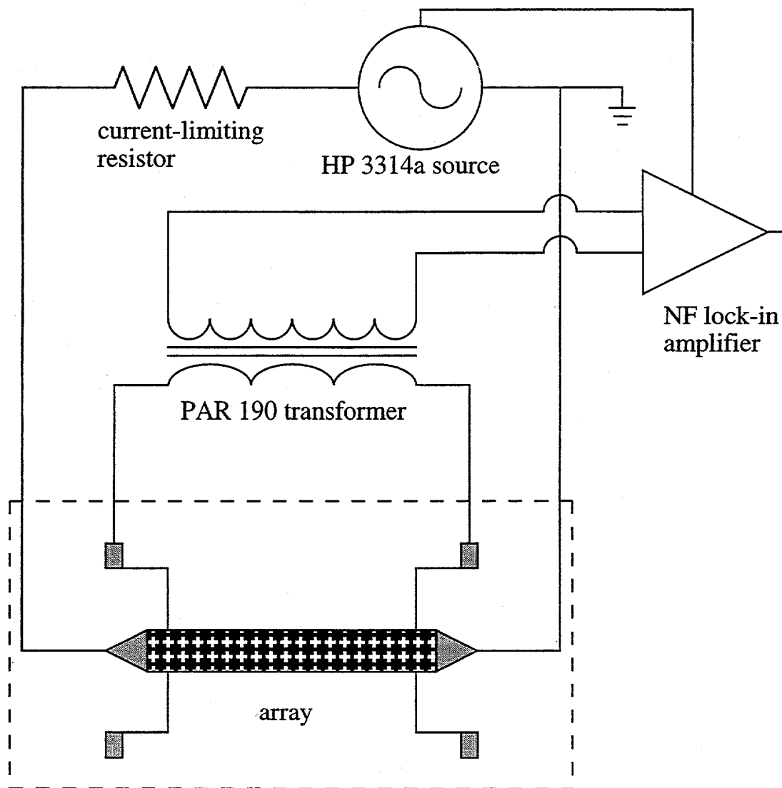
Figure 2.7: Scheme for electrical measurements of arrays.
