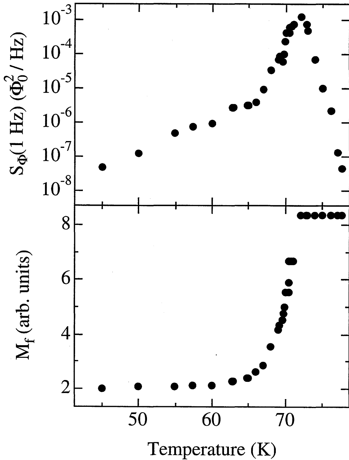
Figure 3.5: (a) S_{\Phi}(1 \text{ Hz}) versus temperature and (b) M_f versus temperature of a 1500 Å-thick film of BSCCO.
