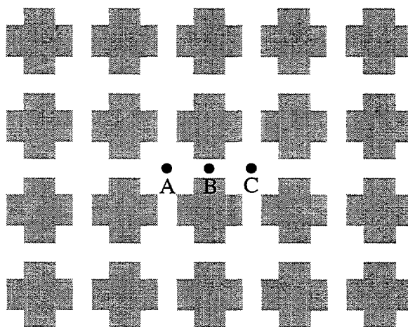
Figure 4.10: Illustration of a vortex moving from the center of an array cell at position A to the center of the adjacent cell at position C while crossing the energy barrier at position B.
