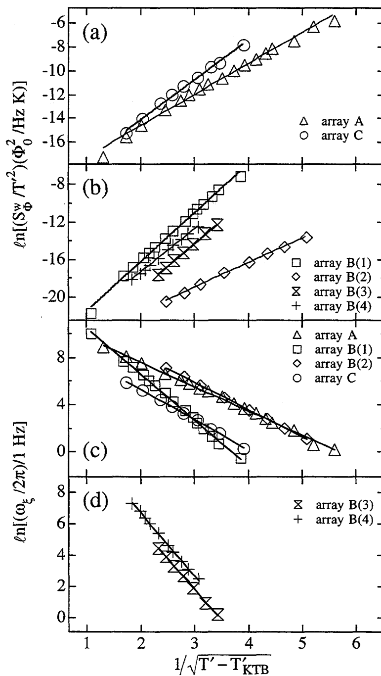
Figure 4.7: (a) and (b) \ln(S_{\Phi}^w/T'^2) versus 1/\sqrt{T' - T'_{\text{KTB}}} of the noise data shown in Fig. 4.4. Values of 2b extracted from the straight line fits shown are listed in Table 4.4. (c) and (d) \ln(\omega_{\xi}/2\pi)/1 \text{ Hz} versus 1/\sqrt{T' - T'_{\text{KTB}}} of the noise data shown in Fig. 4.4. Values of bz extracted from the straight line fits shown are listed in Table 4.4
