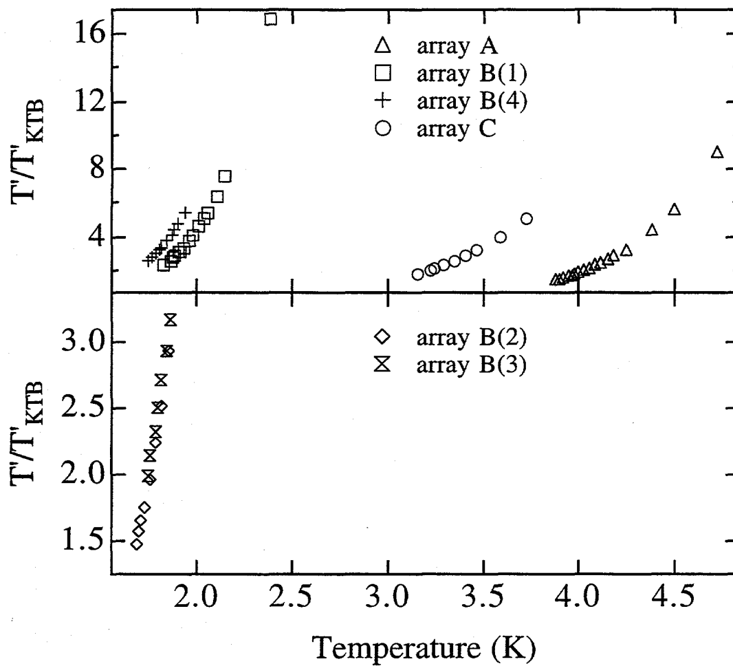
Figure 4.24: T'/T_{KTB} versus temperature for the noise data measurements shown in Fig. 4.4.
