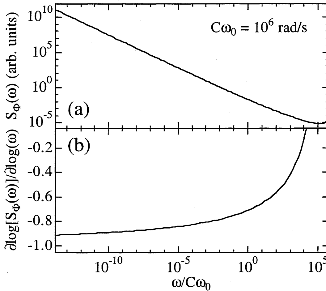
Figure 4.9: (a) S_\Phi(\omega) versus frequency according to Eq. (4.40) with the assumption C\omega_0 = 10^6 rad/s. (b) Slope of S_\Phi(\omega) from part (a) as a function of frequency.
