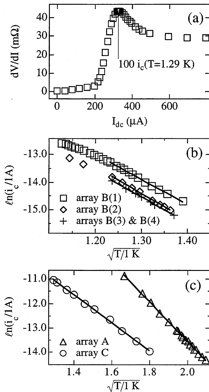
Figure 4.3: (a) dV/dI versus I_{dc} for array B(1), showing N(= 100)i_c(T = 1.29 \text{ K}) . (b) and (c) \ln(i_c) versus \sqrt{T} measured during the experimental runs shown in Fig. 4.4. Values of the slopes and intercepts extracted from the straight line fits shown are given in Table 4.1.
