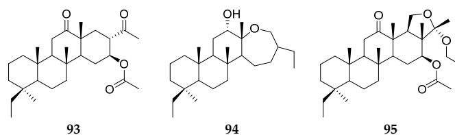
Chart 6. Chemical structures of secondary metabolites (93–95) from P. madagascarensis .
