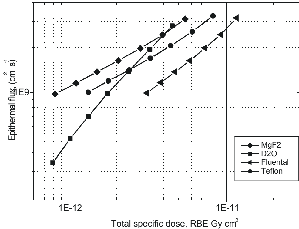
Fig. 1. The computed results obtained in investigations for readily available moderator materials: namely, heavy water, magnesium fluoride, polytetrafluoroethylene and Fludental®.
