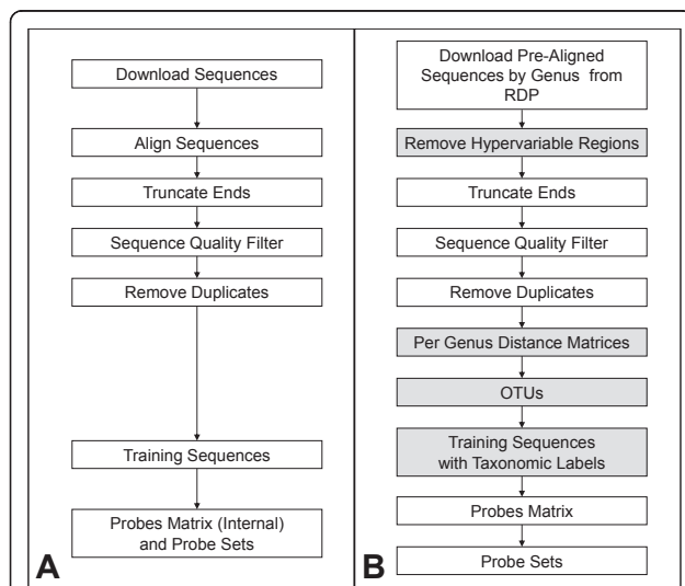
Figure 1 Diagrams of the new and original processing pipelines. Shown are the A) original processing pipeline and B) new processing pipeline for training sequences. The four main differences (shaded boxes) in the new are 1) sequences have their hypervariable regions removed, 2) distance matrices allow 3) grouping ( \leq 1\% sequence difference) into Operational Taxonomic Units (OTUs), and 4) sequences are labelled with their taxonomic designations, as supplied by the Ribosomal Database Project (RDP).
