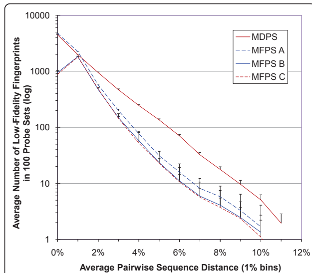
Figure 5 Average pairwise sequence distance metric. This metric focuses on how inaccurate a probe set's low-fidelity fingerprints are. Lower scores are better. The graph was constructed as follows. For each low-fidelity distinct fingerprint of a probe set, the average pairwise sequence difference between its underlying DNA sequences was determined. A count of how many fingerprints within each binned (1% increments) average was kept. Each point represents the average count of each bin for 100 probe sets. MFPS A (OTU and genus penalties set to 1 and 0, respectively) is superior to MDPS except for having a few more fingerprints from 0% to 1%; scores in this range are from highly similar sequences but from OTUs in different genera. MFPS B (OTU and genus penalties set to 1 and 30, respectively) shows further improvement in distances greater than 1%, but unlike MFPS A or MDPS, has markedly fewer low-fidelity distinct fingerprints with sequence distances from 0% to 1%. The improvement in distances greater than 1% is the same windfall seen in HFR scores when the genus-level penalty was set to 30 (see Figure 3). MFPS C (OTU and genus penalties set to 1 and 200, respectively) shows only a small improvement over MFPS B. Error bars (showing upper bars only for better visibility) are standard deviations from 100 probe sets.
