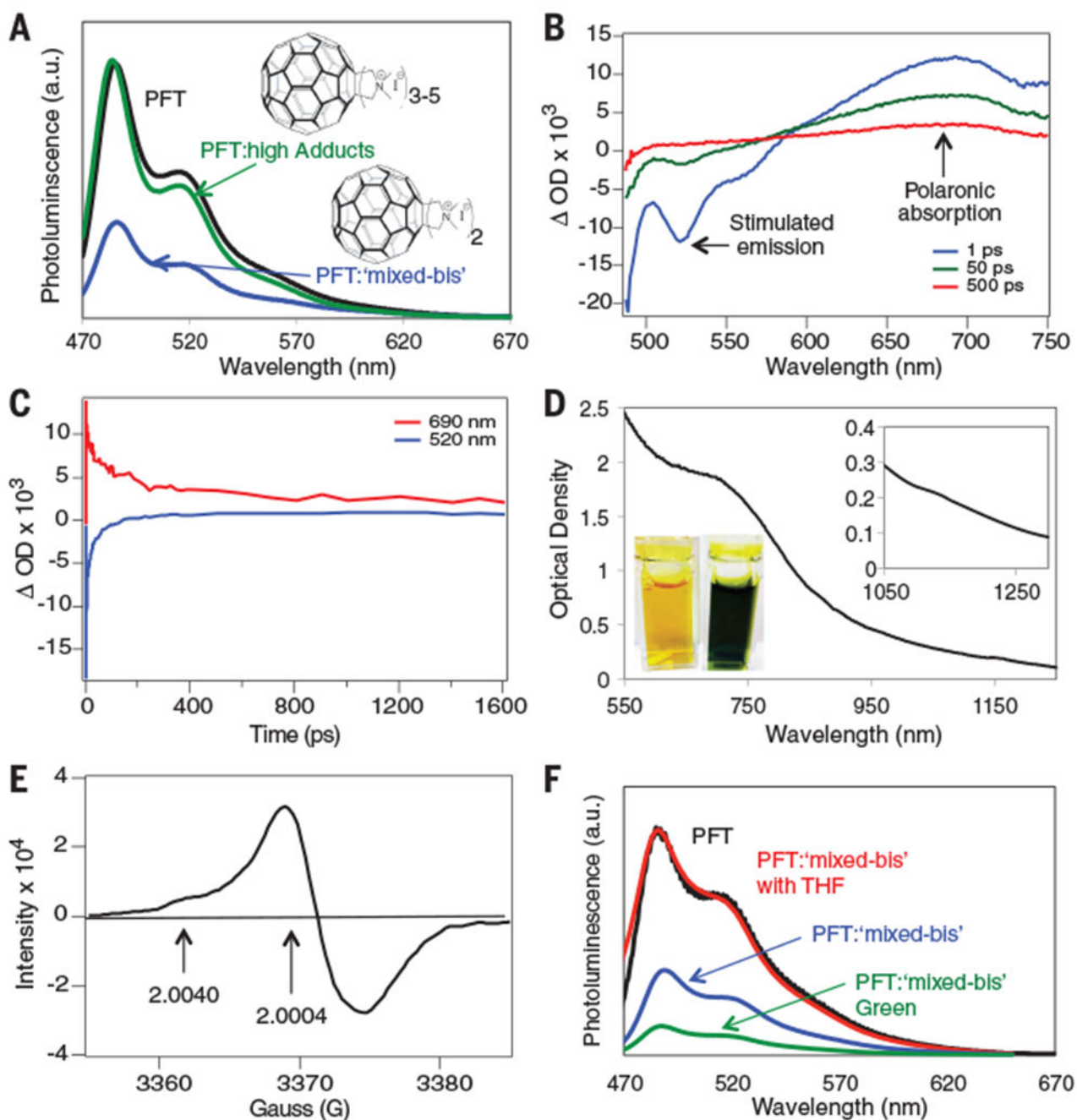
Fig. 3. Formation of P^+ and N^- polarons requires intimate assembly of the polymer and fullerene.
