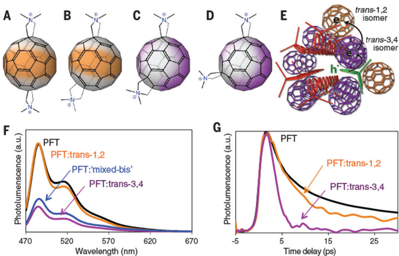
Fig. 4. Spectroscopic evidence for long-lived charged species in solution.
