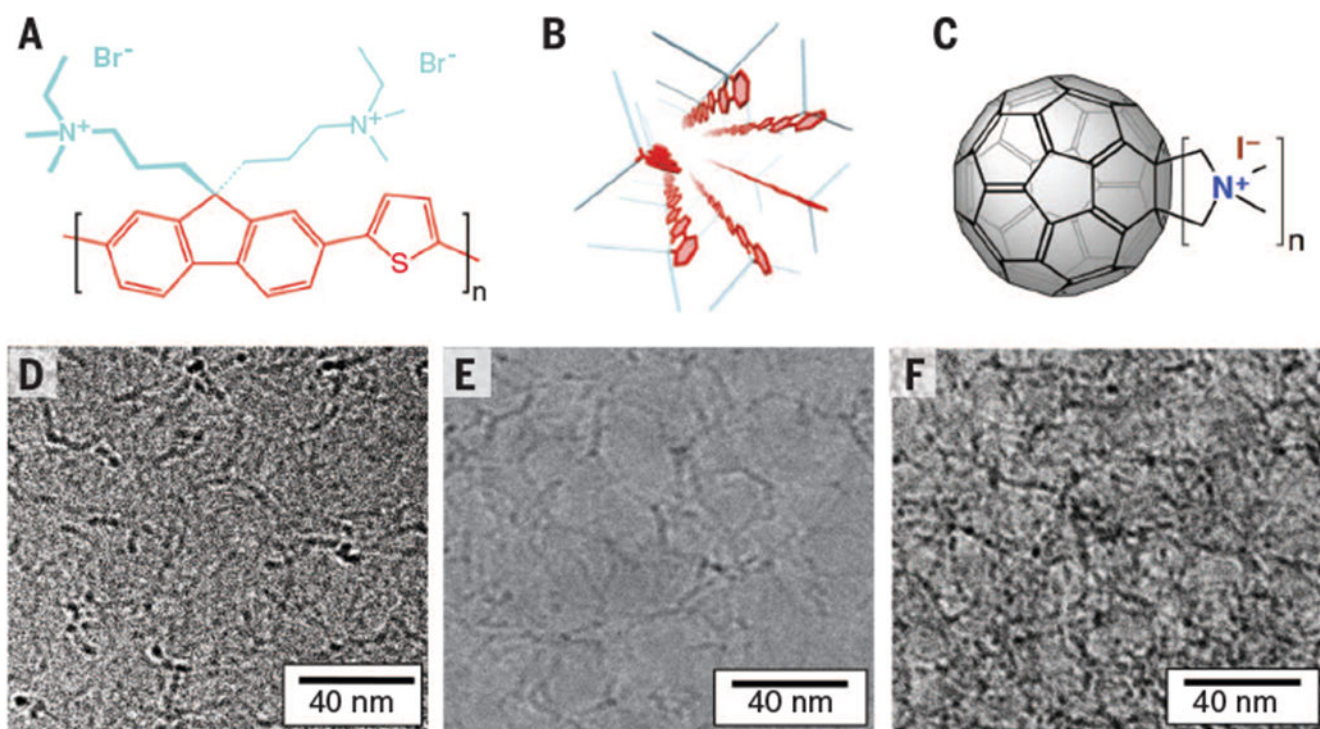
Fig. 1. PFT and charged fullerene structure and assembly.
