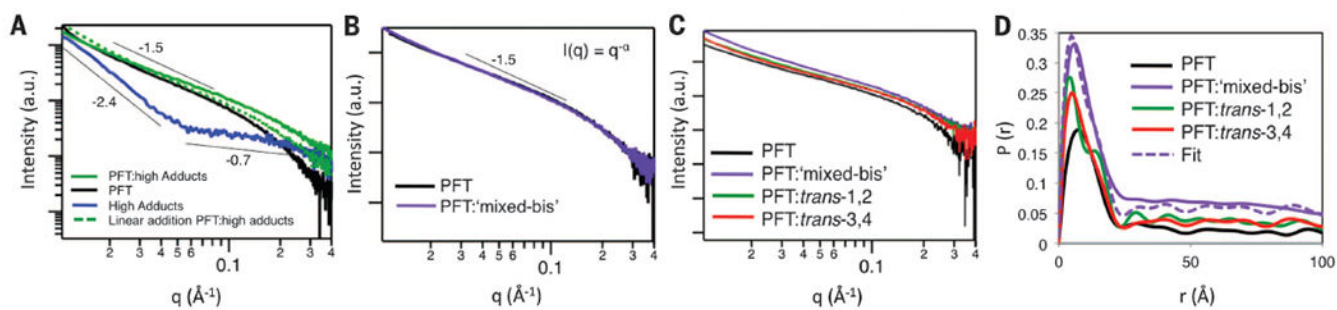
Fig. 2. SAXS data for PFT and PFT/fullerene mixtures.
