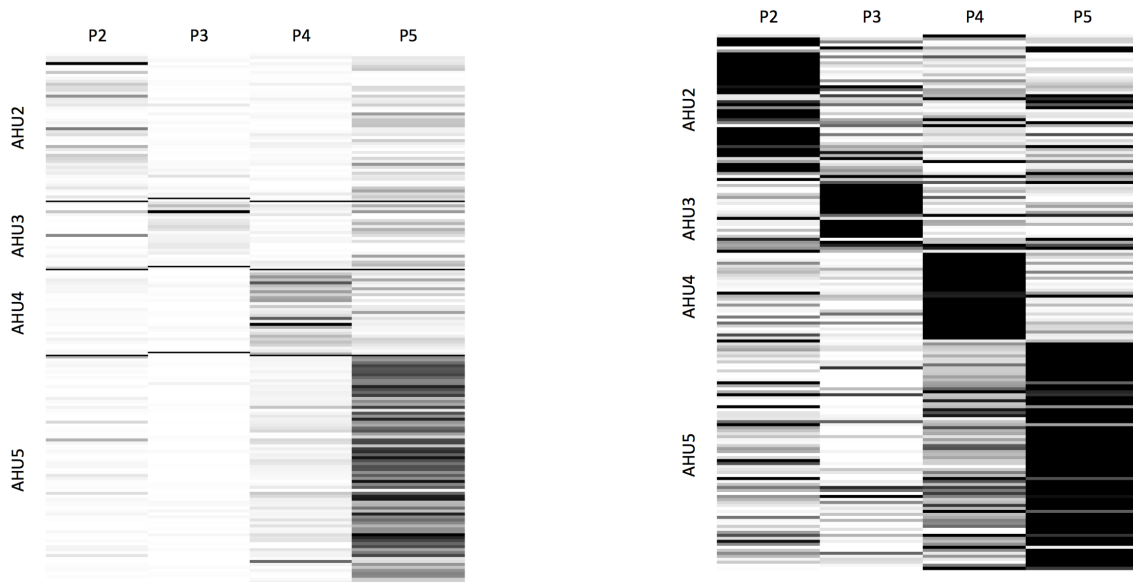
(b) Application of voting across perturbation periods. Our metric – the deviation magnitude of the vector — is normalized for each zone across its values for the different perturbation periods, and not against all other zones.
