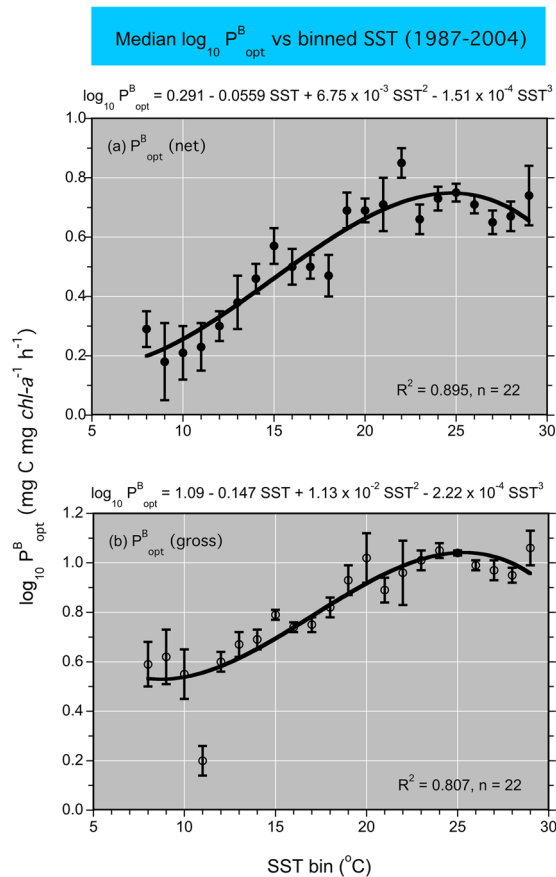
Figure 5. (a,b) Relationships of \log_{10} P_{\text{opt}}^B (net) and (gross) to binned sea-surface temperature (SST). Time-series observations included additional measurements from 2002 to 2004 to update three-order polynomial regressions of Son et al. 31 .
