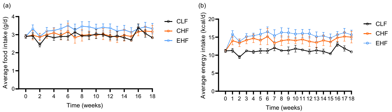
Fig. 1. Food intake (a) and energy intake (b) of male C57BL/6J mice fed experimental diets: control low-fat diet (CLF, 10 % kcal from fat), control high-fat diet (CHF, 45 % kcal from fat) and high-fat diet with TVA and RA-enriched tallow (EHF, 45 % kcal from fat) for 19 weeks. Body weight ( n 12/group) and energy intake ( n 12/group) were measured weekly during the feeding period. Values are expressed as mean \pm standard deviation. TVA, trans vaccenic acid; RA, rumenic acid.
