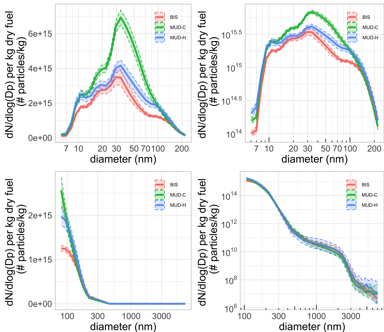
Figure 5.6: Particle size distribution for fine (diameter <math><2.5\text{ mm}</math>) and ultrafine (diameter <math><1000\text{ nm}</math>) particle number concentrations per kilogram of dry fuel consumed for the BIS ( n = 13 ), cold-start mud chulha (MUD-C, n = 15 ), and hot-start mud chulha (MUD-H, n = 10 ) tests (bringing 5 L of water to boil) measured by the FMPS (top left and top right lots) and the OPS (bottom left and bottom right plots). Shaded bands represent 95% confidence bounds. Note that plots on the left are plotted on a normal-log scale and plots on the right are plotted on a log-log scale.
