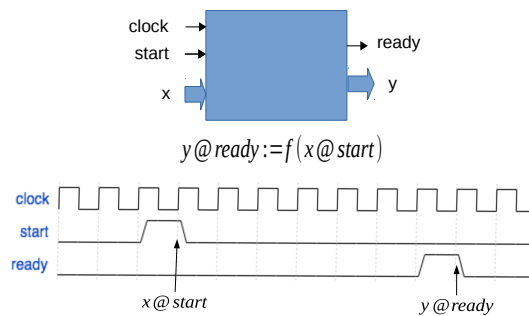
Figure 4.10: Verilog Model
