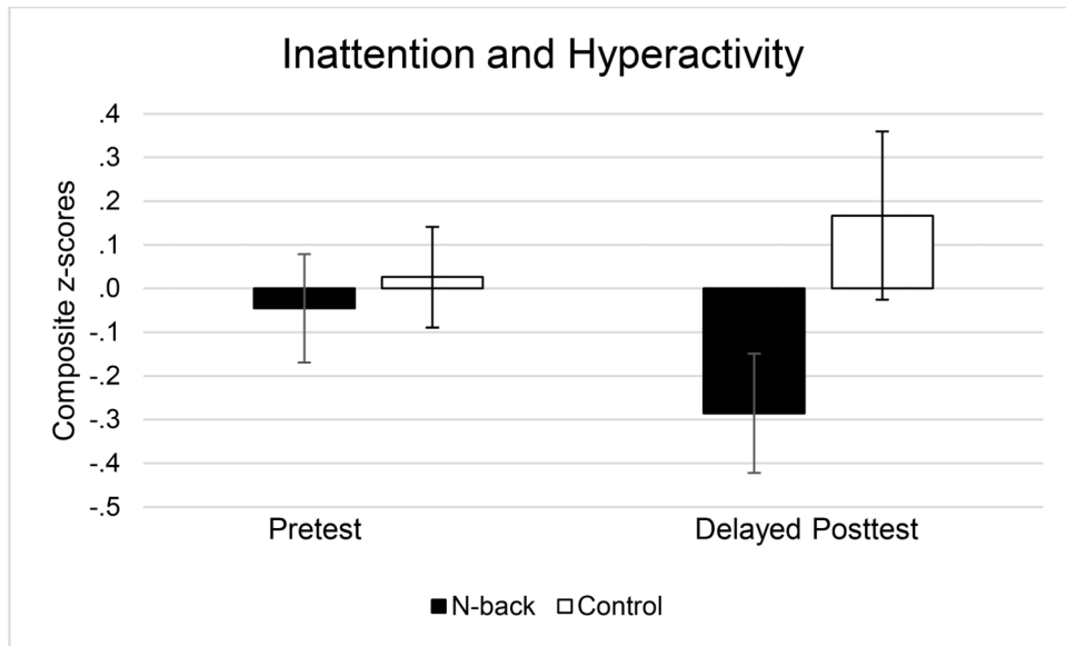
Figure 2: Parent rating of inattention and hyperactivity by training group. Note that better performance is represented by negative numbers (i.e. fewer symptoms). Error bars represent standard errors.
