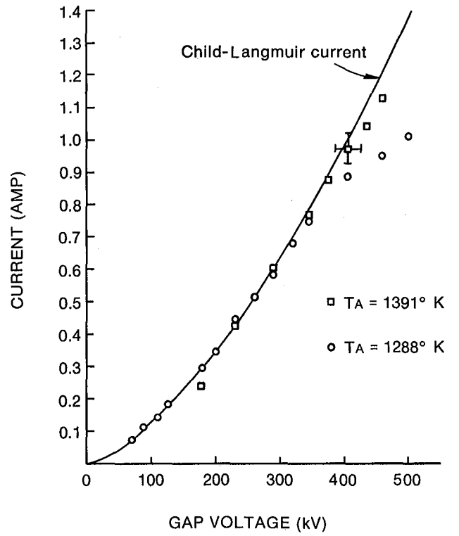
FIG. 4 - CURRENT VS. VOLTAGE APPLIED TO THE ANODE FOR TWO VALUES OF Cs EMISSION.
