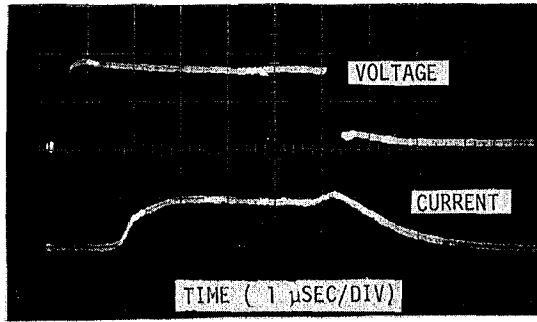
FIG. 2 - TYPICAL VOLTAGE AND CURRENT WAVE FORMS.
