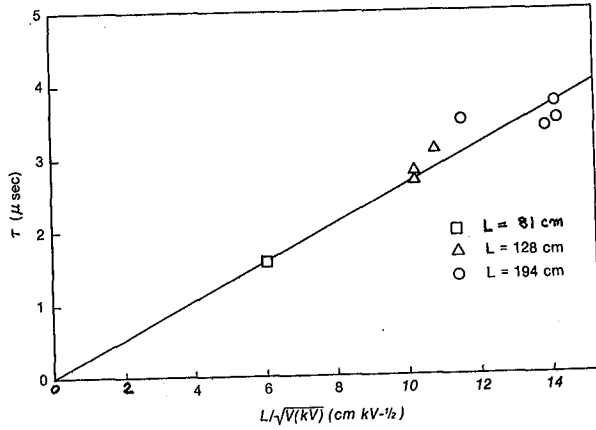
FIG. 3 - TIME OF FLIGHT MEASUREMENTS OF Cs 1+ BEAM. L IS THE DISTANCE OF THE DRIFT SPACE.
