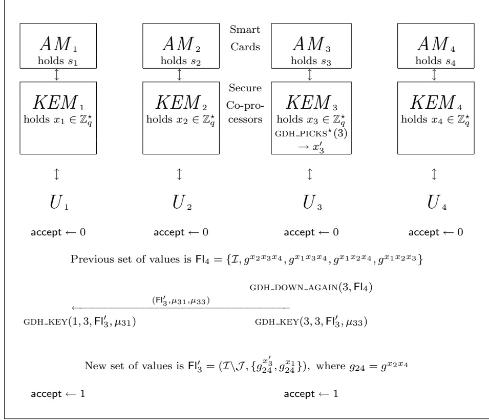
Fig. 5. Algorithm Remove. A practical example with 4 players: \mathcal{I} = \{U_1, U_2, U_3, U_4\} and \mathcal{J} = \{U_2, U_4\} . The new multicast group is \mathcal{I} = \{U_1, U_3\} and GC = U_3 .
