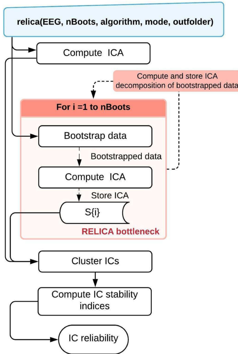
Figure 4. Original RELICA workflow.
