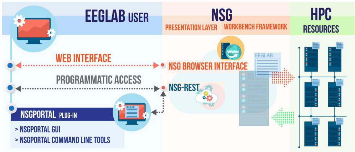
Figure 1. High-level overview of the Open EEGLAB Portal (OEP) workflow.
