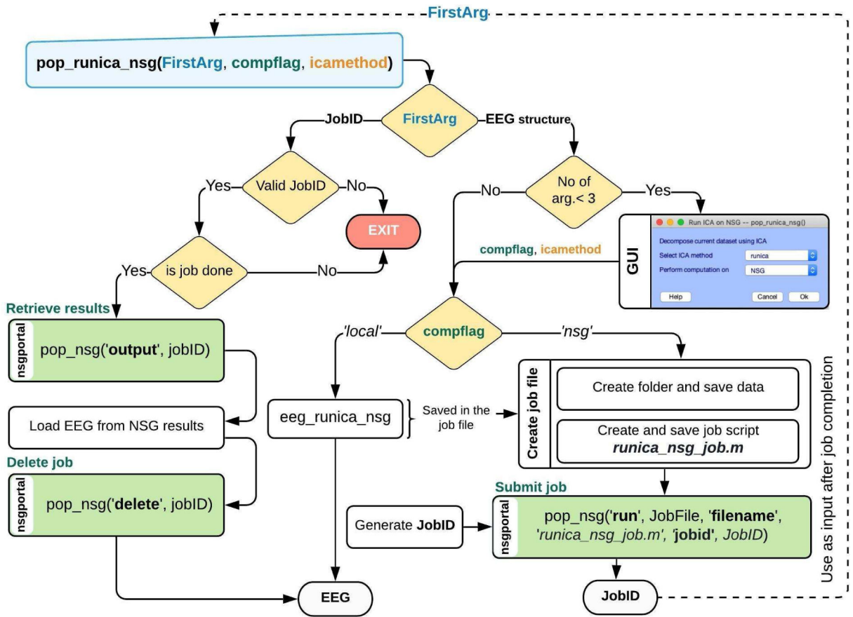
Figure 3. Workflow of the example plug-in RUNICA_NSg.
