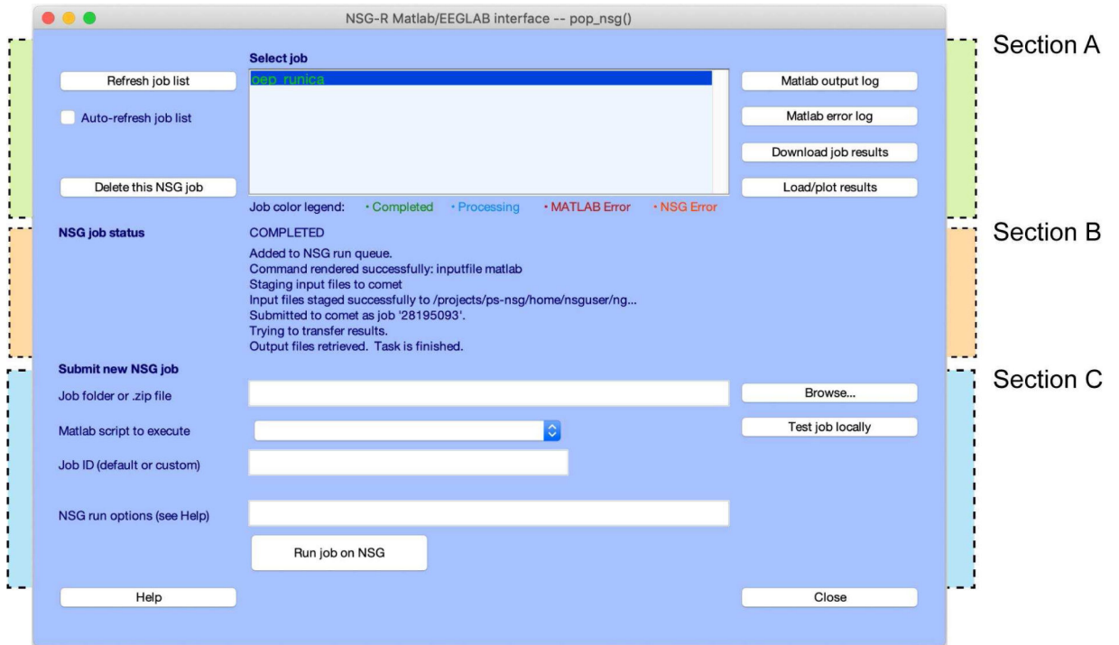
Figure 2. The pop_nsg.m graphical user interface (GUI) window.
