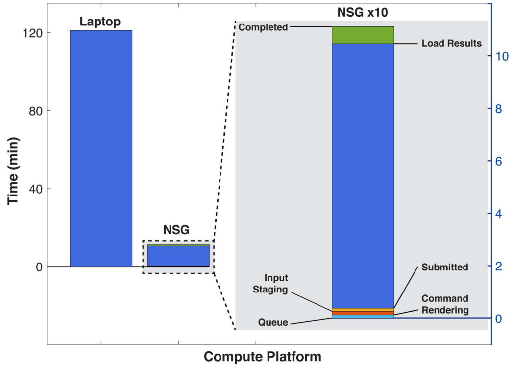
Figure 6. RELICA processing time on NSG versus a laptop.
