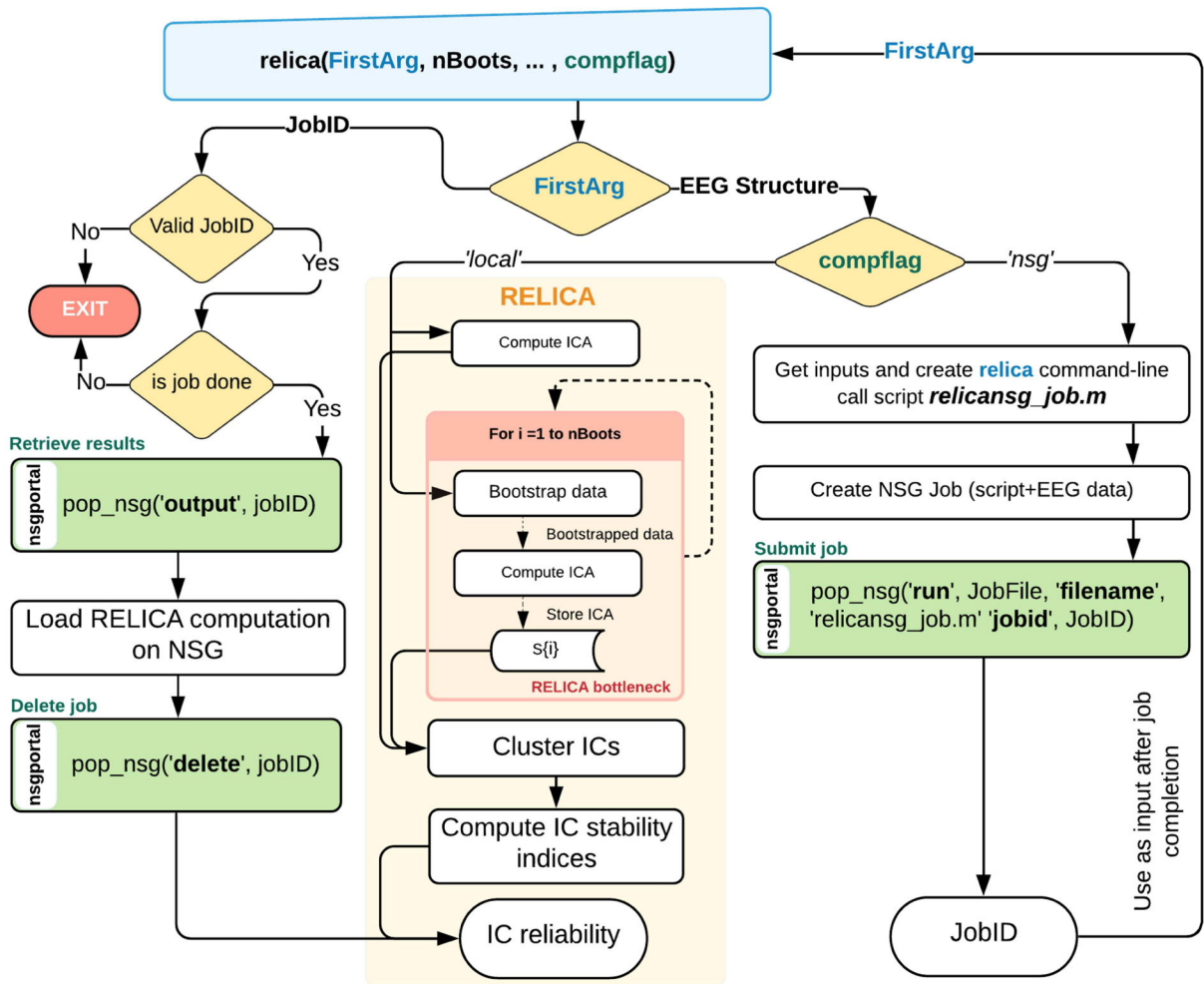
Figure 5. The NSG-capable RELICA plug-in.
