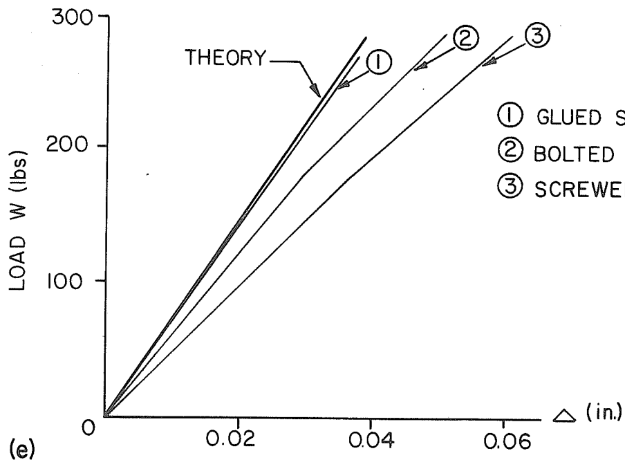
FIG. 2.2 COMPONENT TEST FOR MOMENT CONTINUITY
