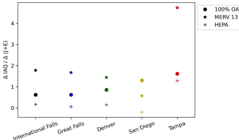
Fig. 17. Marginal improvement in IAQ relative to costs including the cost of CO 2 emissions for the five locations.
