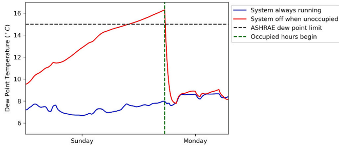
Fig. 2. Dew point temperature in the core zone for the system in Tampa on August 25–26.
