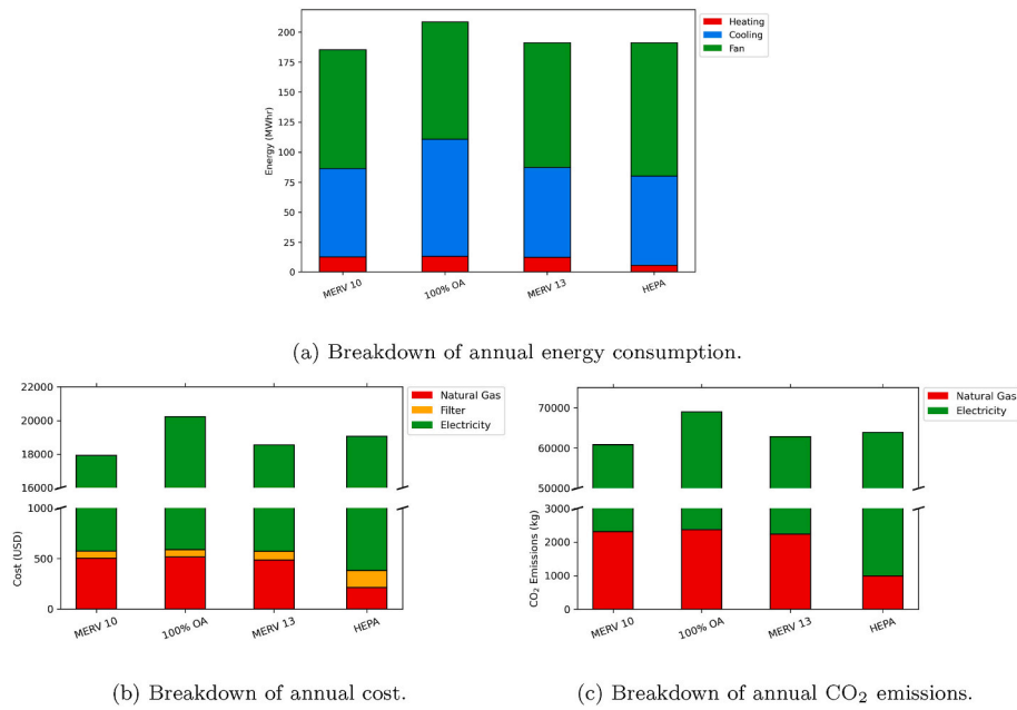
Fig. 8. Annual energy, cost and CO 2 emission results for Tampa.
