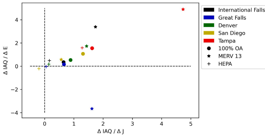
Fig. 16. Marginal improvement in IAQ relative to costs and CO 2 emissions for the five locations.
