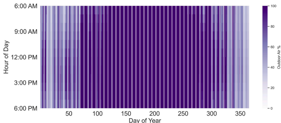
Fig. 7. Dynamic usage of outdoor air in International Falls for the 100% outdoor air strategy.
