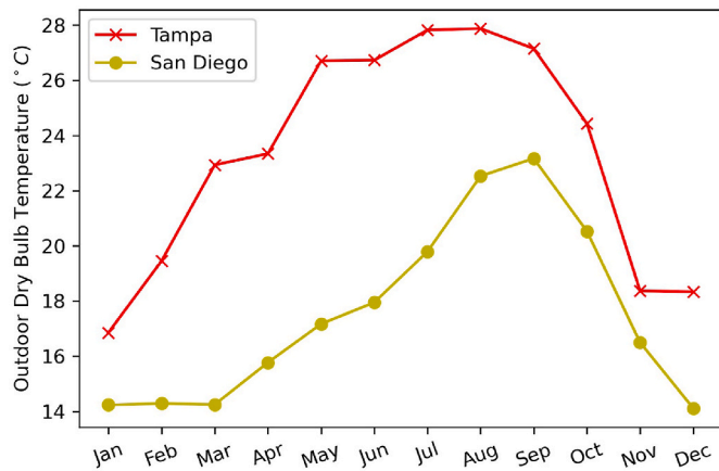
Fig. 11. Average monthly temperatures in Tampa and San Diego.
