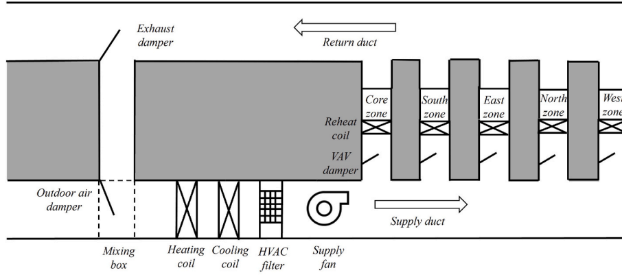
Fig. 1. Schematic of VAV system servicing the bottom floor of the five zone medium office building.
