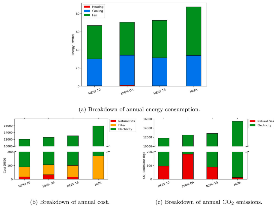
Fig. 9. Annual energy, cost and CO 2 emission results for San Diego.
