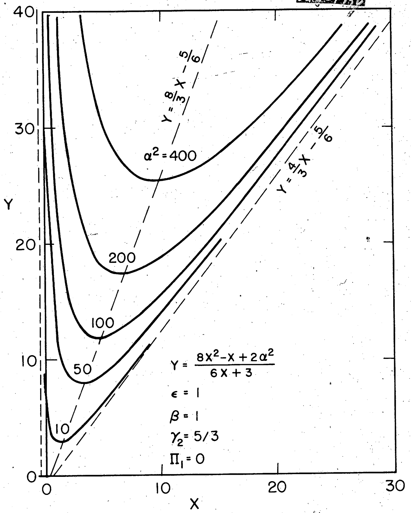
Plots of Y(X) , Eq.(16), for various \alpha^2 , and of Eqs. (21) and (31).
