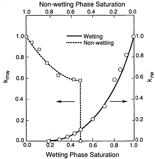
Figure 7. Simulated wetting and nonwetting phase relative permeabilities for the lognormal aperture distribution of Figures 2 and 4 with long-range anisotropic spatial correlation.
