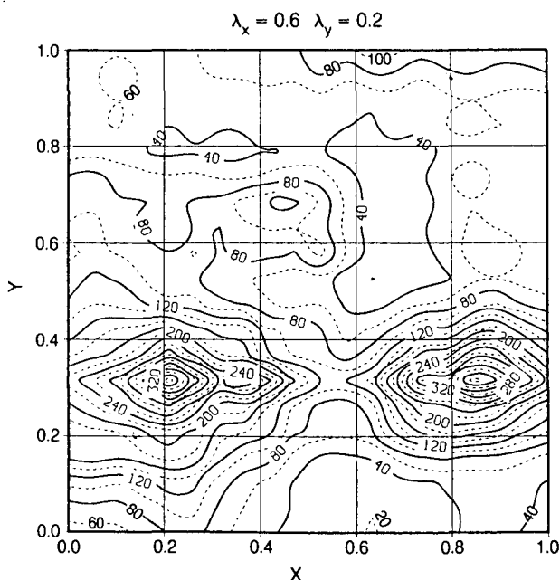
Figure 2. A lognormal aperture distribution with anisotropic spatial correlation (Case 2, Table 1).
