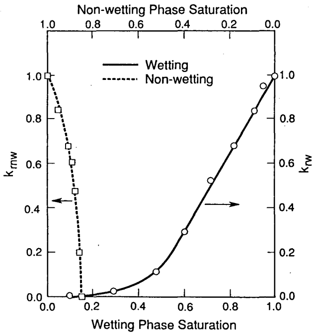
Figure 6. Simulated wetting and nonwetting phase relative permeabilities for the lognormal aperture distribution of Figures 1 and 3.
