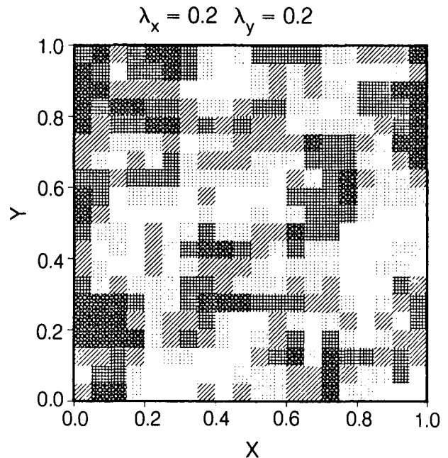
Figure 3. A 20 x 20 discretized version of the fracture apertures shown in Figure 1. Lighter shading corresponds to larger apertures.
