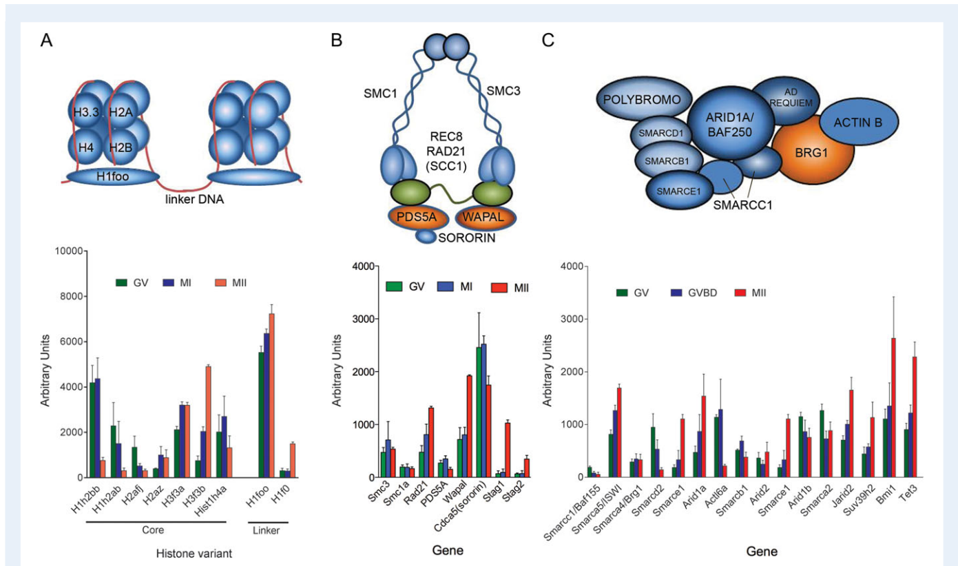
Figure 3 Dynamic changes in components of the chromatin during oocyte maturation due to contrasting patterns of components translation. Schematic representation of the components of the nucleosome, cohesins, and the chromatin switch/sucrose non-fermentable (SWI/SNF) complex are reported on top. The lower panel reports the level of mRNAs bound to polysomes for the above components as well as additional chromatin remodelers thought to function at the maternal to zygote transition. The data are derived from deposited data (GEO dataset Accession: GSE35106 ID:200 035 106). SMC1: Structural Maintenance Of Chromosomes 1; SMC3: Structural Maintenance Of Chromosomes 3; REC8: REC8 Meiotic Recombination Protein; RAD21: Rad21 (S.Pompe) Homolog (Scc1); SCC1: alternative name for RAD21 (used interchangeably); PDS5A: Cohesin Associated Factor A; WAPAL: Wings Apart-Like Homolog; SORORIN: Cell Division Cycle-Associated Protein 5 (CDCA5); STAG1: Stroma Antigen 1; STAG2: Stromal Antigen 2; POLYBROMO1: BRG1-Associated Factor 180 (Baf180); SMARCD1: SWI/SNF Related, Matrix Associated, Actin Dependent Regulator Of Chromatin, Subfamily D, Member 1; SMARCB1: SWI/SNF Related, Matrix Associated, Actin Dependent Regulator Of Chromatin, Subfamily B, Member 1; SMARCE1: SWI/SNF Related, Matrix Associated, Actin Dependent Regulator Of Chromatin, Subfamily E, Member 1; SMARCC1: SWI/SNF Related, Matrix Associated, Actin Dependent Regulator Of Chromatin Subfamily C Member 1; ARID1A: AT-Rich Interaction Domain 1A (BAF250); AD REQUIEM: Double PHD Fingers 2; BRG1: Brahma-related gene-1 (known as SMARCA4); SMARCA4: SWI/SNF Related, Matrix Associated, Actin Dependent Regulator Of Chromatin, Subfamily A, Member 4 (BRG1); SMARCA5: SWI/SNF Related, Matrix Associated, Actin Dependent Regulator of Chromatin, Subfamily A, Member 5; SMARCD2: SWI/SNF Related, Matrix Associated, Actin Dependent Regulator Of Chromatin, Subfamily D, Member 2; ACT16A: Actin Like 6A; ARID2: AT-Rich Interaction Domain 2; ARID1B: AT-Rich Interaction Domain 1B; SMARCA2: SWI/SNF Related, Matrix Associated, Actin Dependent Regulator Of Chromatin, Subfamily A, Member 2; JARID2: Jumonji And AT-Rich Interaction Domain Containing 2; SUV39H2: Suppressor Of Variegation 3–9 Homolog 2; BMI1: Polycomb Ring Finger Proto-Oncogene; TET3: Tet Methylcytosine Dioxygenase 3.
