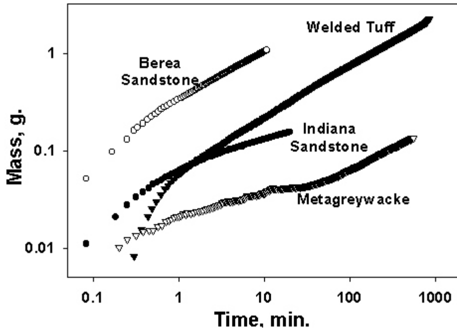
Figure 1. Experimental results showing cumulative imbibition into Berea sandstone, Indiana sandstone, welded tuff, and metagreywacke.
