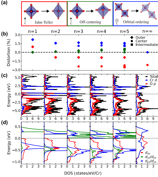
FIG. 6. Relevant distortions of the \text{CrO}_6 octahedra for spin-polarized calculations and calculated density of states (DOS) across the series. (a) Sketch of the out-of-plane Jahn-Teller distortion, off-centering of the chromium atoms, and in-plane Jahn-Teller distortion associated with spin-orbital ordering. (b) Amplitude of each of the distortions in the different layers, where the colors correspond to the boxes in (a). (c) The total and site-projected density of states. (d) The orbital projected density of states. The blue and green d_{xz}/d_{yz} correspond to the DOS of the d_{xz} or d_{yz} orbitals (alternating in each layer).
