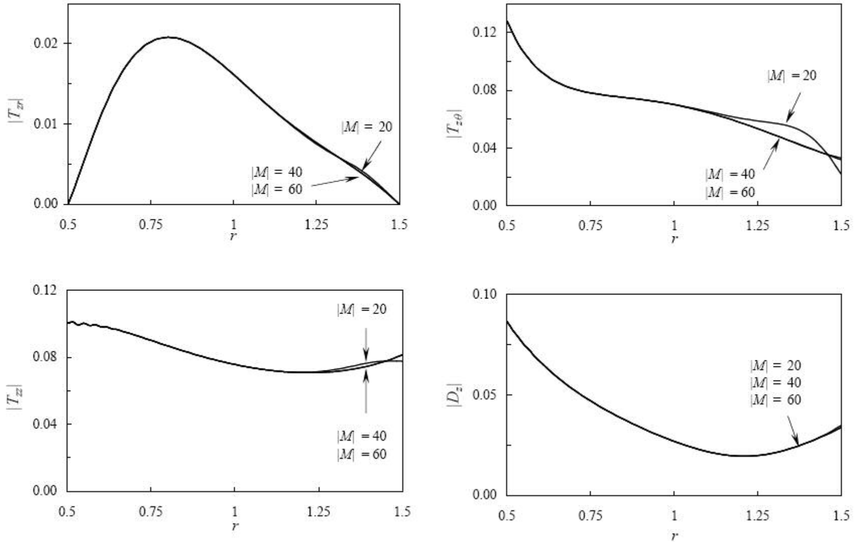
Figure 5(b). Comparison of Generalized Stresses of Green Function for Homogeneous PZT-4 cylinder Due to Unit Radial Force, Opened-Opened Circuit Conditions.
