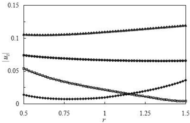
Figure 11. Generalized Displacements For a 2-layered Piezoelectric Cylinder due to a Point Load ( —□— : Radial Load, —◇— : Circumferential Load, —△— : Axial Load, —○— : Point Charge).
