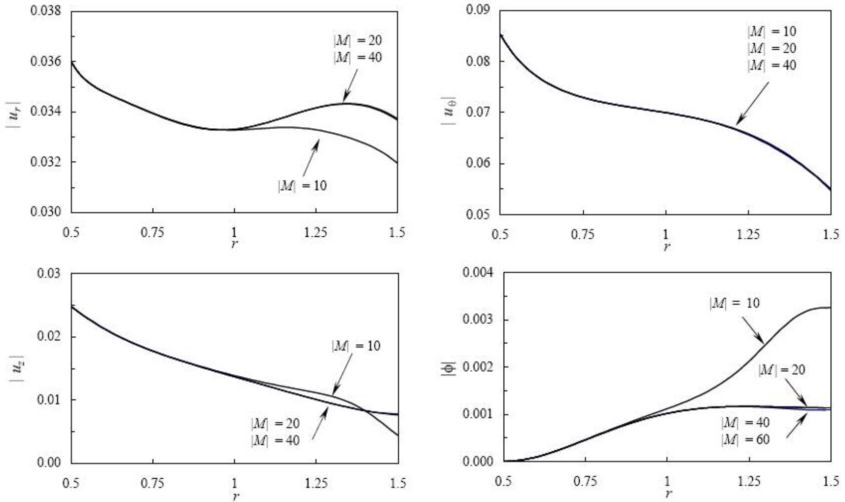
Figure 5(a). Comparison of Generalized Displacements of Green Function for Homogeneous PZT-4 cylinder Due to Unit Radial Force, Opened-Opened Circuit Conditions.
