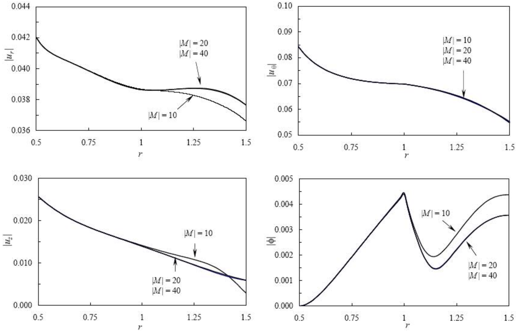
Figure 10(a). Generalized Displacements of Green Function for a 2-layer Opened-Opened Piezoelectric Cylinder due to a Radial Point Load on the Outer Surface.
