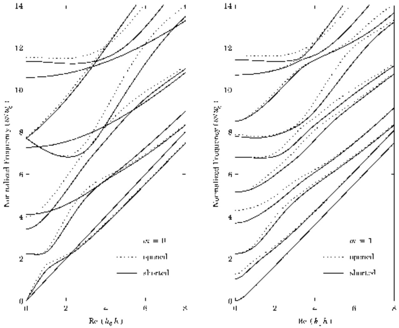
Figure 3. Frequency Spectra Comparison Between Opened-Opened and Shorted-Shorted Circuit Conditions for m=0 and m=1 .
