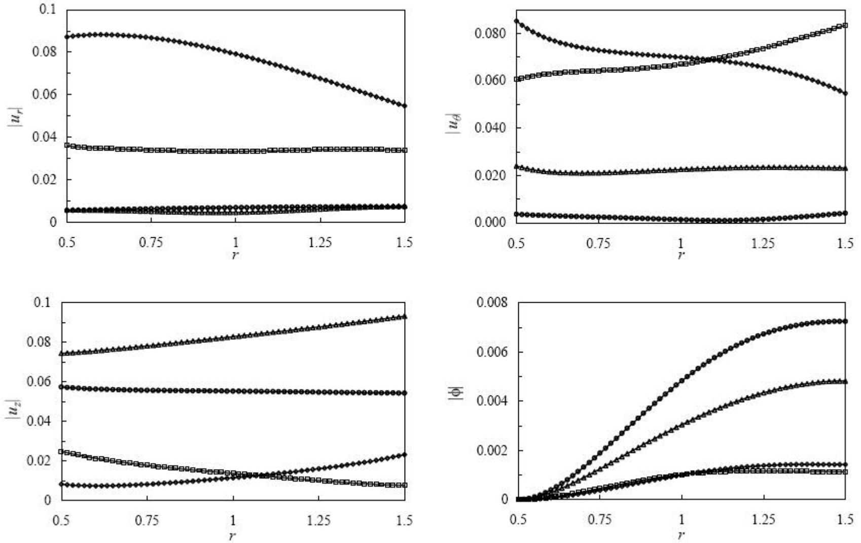
Figure 6. Generalized Displacements in an Opened-Opened Cylinder along (r, \pi/4, h/4) due to External Loads Applied at (r_{out}, 0, 0) for \omega = 1.5 ( \square : Radial Load, \diamond : Circumferential Load, \triangle : Axial Load, \circ : Point Charge).
