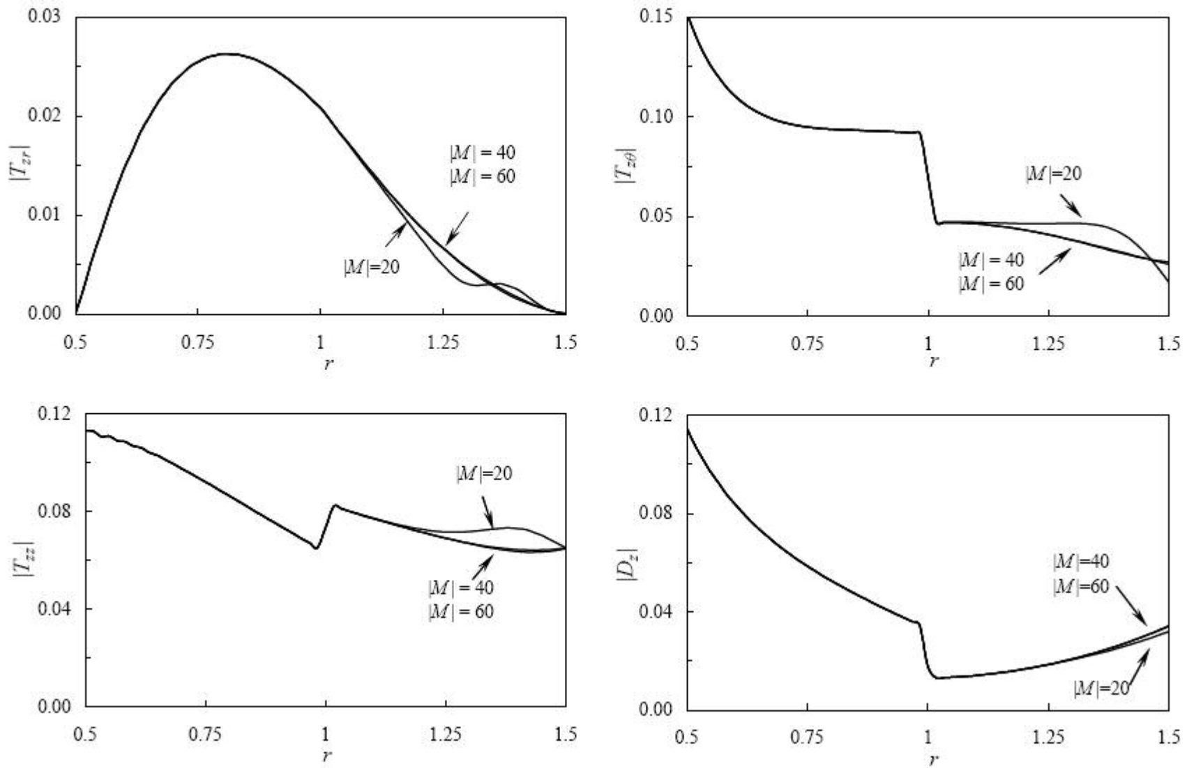
Figure 10(b). Generalized stresses of Green Function for a 2-layer Opened-Opened Piezoelectric Cylinder due to a Radial Point Load on the Outer Surface.
