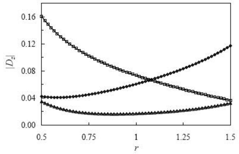
Figure 9. Generalized Stresses in a Shorted-Shorted Cylinder along (r, \pi/4, h/4) due to External Loads Applied at (r_{out}, 0, 0) for \omega = 1.5 ( —□— : Radial Load, —◇— : Circumferential Load, —△— : Axial Load, —○— : Point Charge).
