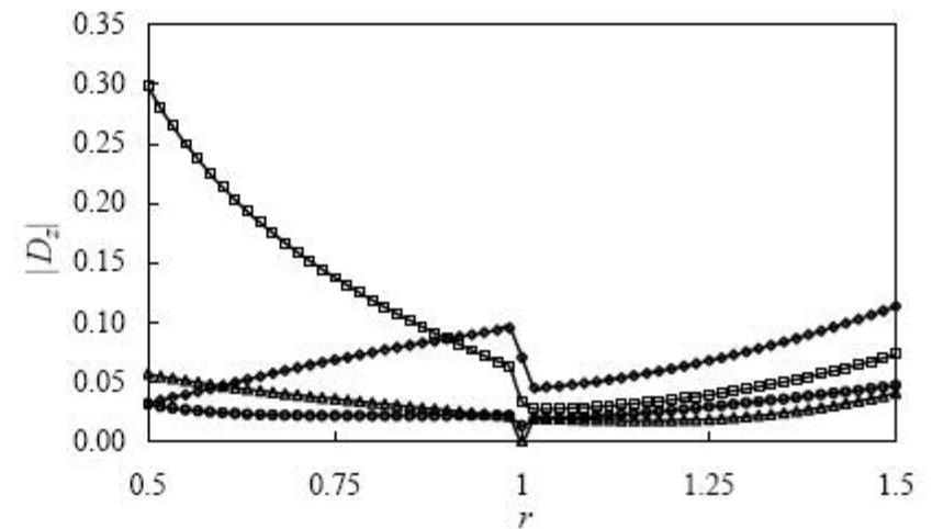
Figure 12. Generalized Stresses For a 2-layered Piezoelectric Cylinder due to a Point Load (—□— : Radial Load, —◇— : Circumferential Load, —△— : Axial Load, —○— : Point Charge).
