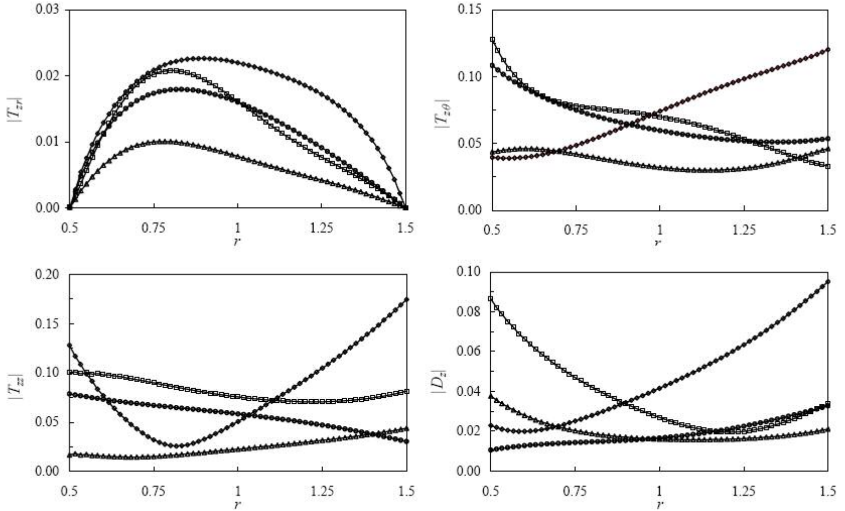
Figure 7. Generalized Stresses in an Opened-Opened Cylinder along (r, \pi/4, h/4) due to External Loads Applied at (r_{out}, 0, 0) for \omega = 1.5 (—□— : Radial Load, —◇— : Circumferential Load, —△— : Axial Load, —○— : Point Charge).
