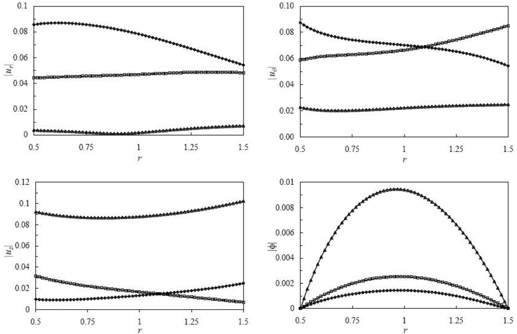
Figure 8. Generalized Displacements in a Shorted-Shorted Cylinder along (r, \pi/4, h/4) due to External Loads Applied at (r_{out}, 0, 0) for \omega = 1.5 (—□— : Radial Load, —◇— : Circumferential Load, —△— : Axial Load, —○— : Point Charge).
