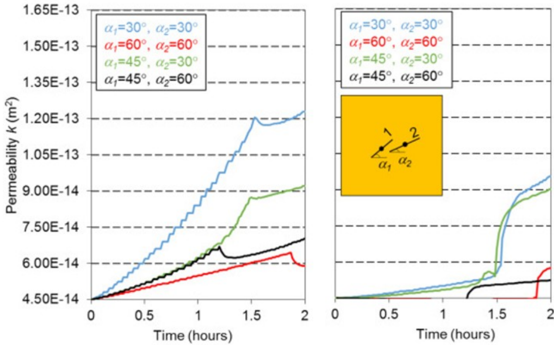
Fig. 11. Variation with time (hours) of the permeability ( \text{m}^2 ) of in the centre of the fractures 1 (left) and 2 (right) in rock domain FD2 obtained for fracture angles \alpha_1 and \alpha_2 (results obtained at 2 h of injection).
