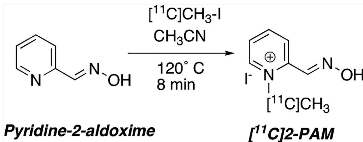
Scheme 2. Radiosynthesis of Tracer [ 11 C]2-PAM
