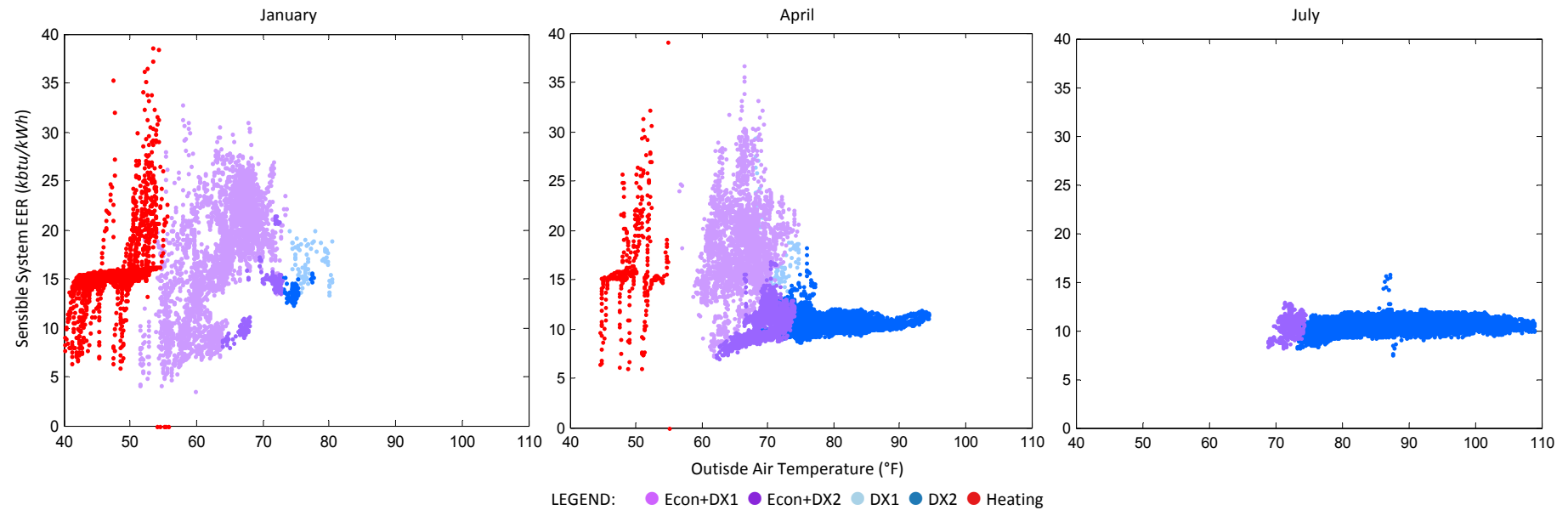
FIGURE 8: SENSIBLE SYSTEM EFFICIENCY IN EACH MODE OF OPERATION FOR THREE DIFFERENT SEASONS. DATA FOR ONE MONTH PERIODS IN ONE MINUTE INTERVALS.
